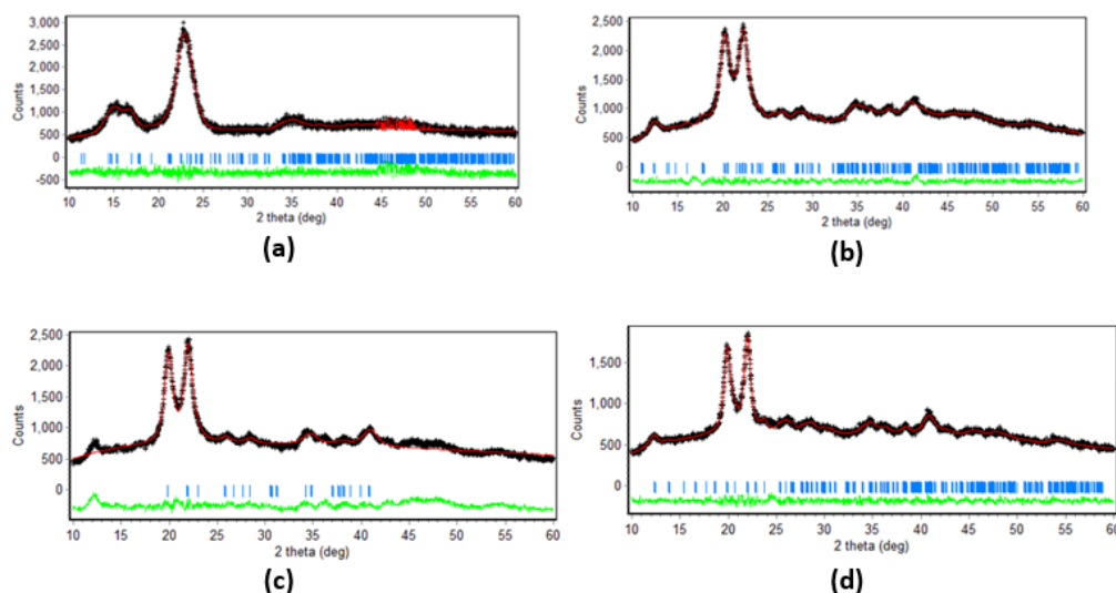
Figure 4. XRD refinement of (a) cotton (b) acid concentration observation (c) reaction temperature observation and (d) reaction time observation by using Rietica software, Le Bail method. Symbol of (+) represents data observation of XRD, red line represents calculation results, vertical blue line represents expected Bragg position and green line represents the difference between observation and calculation data.
