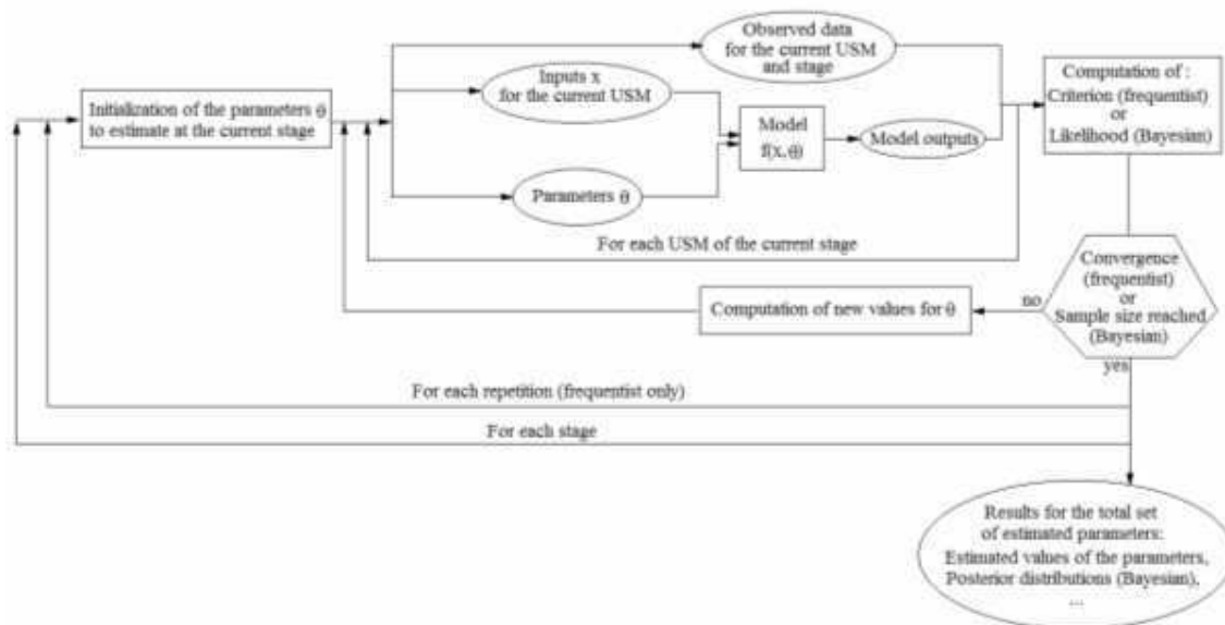
Figure 5 : Parameter estimation process implemented in the software. USM stands for SYMU.
