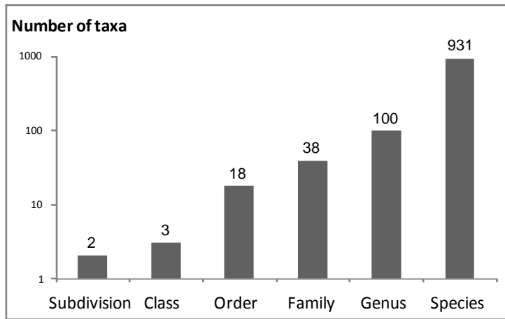
Figure 22: Number of taxa for each taxonomic resolution
