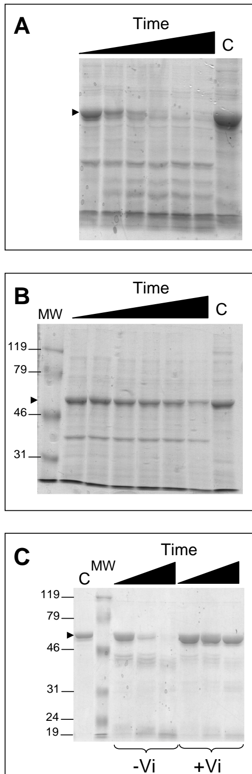
Figure 2. SDS-PAGE of BmrA-enriched membranes or BmrA purified in DDM and after limited proteolysis with trypsin. BmrA in membranes in the apo conformation ( A ) or in the vanadate-inhibited conformation ( B ) and after incubation with trypsin for 5 min, 15 min, 30 min, 1 h, 2 h and 3 h (from left to right lanes); ( C ) BmrA purified in detergent in the apo conformation (lanes 3-5), and in the vanadate-inhibited conformation (lanes 6-8) and after incubation with trypsin for 5, 15 and 30 min (from left to right lanes). C is the control lane with no trypsin added with the black arrowhead showing the position of the full-length BmrA. The masses of the molecular weight markers (MW) are indicated in kDa.
