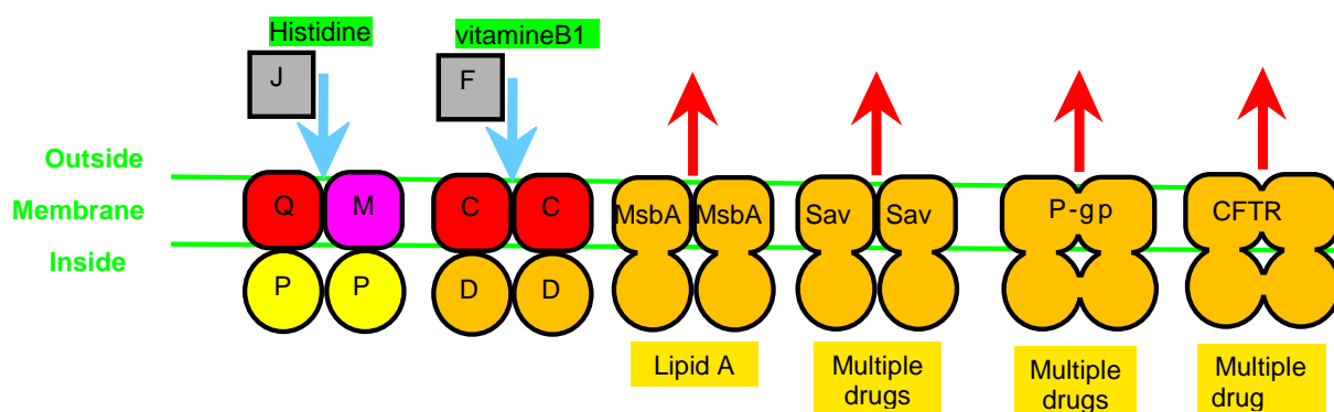
Figure 14. Core structure of ABC transporters
