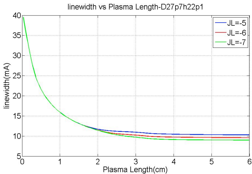
Figure 4-4-11: Same as Fig. 4-4-8, but kTe=300 \text{ eV} , kTi=200 \text{ eV} ; Ne=5 \times 10^{20} \text{ cm}^{-3} ; \Delta\lambda_D=27.7 \text{ mÅ} , \Delta\lambda_h=22.1 \text{ mÅ} ; \Delta\lambda_{tot}=40.9 \text{ mÅ} .
