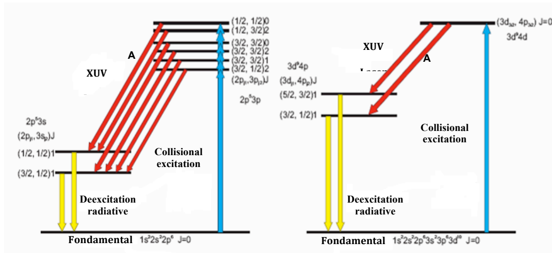
Figure 1-2: Diagram of pumping by collisional excitation. Left) neon like ion, the transition A is the most intense among the six possible transitions. Right) nickellike ion. Transition A is more intense for atoms of high atomic number [28].
