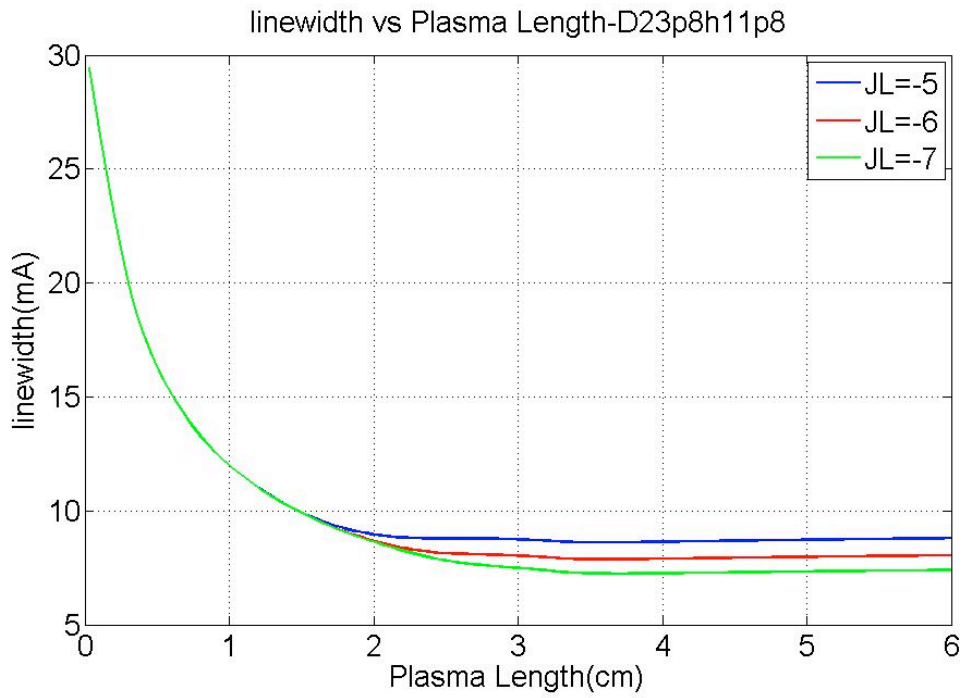
Figure 4-4-8: Amplified linewidth as a function of plasma length: kT_e = 200 eV, kT_i = 150 eV; Ne = 2 \times 10^{20} \text{ cm}^{-3} ; \Delta\lambda_D = 23.8 mÅ, \Delta\lambda_h = 11.8 mÅ; \Delta\lambda_{tot} = 30.5 mÅ
