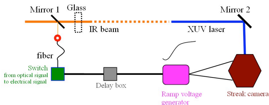
Figure 4-5-1. sketch of the streak camera triggering beamline
