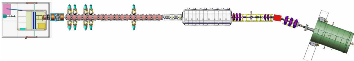
Figure 1.13: Sketch of the LIPAc accelerator [35].
