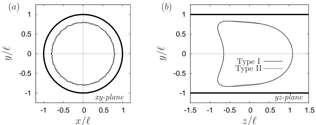
Figure 2.9: Comparisons of steady capsule profiles of different mesh sizes. (a) Cross-sectional profiles on xy -plane; (b) Longitudinal profiles on yz -plane. Ca = 0.05 , a/\ell = 0.9 , NH membrane, cylindrical channel.
