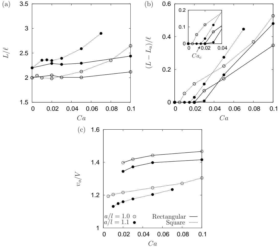
Figure 3.4: Effect of Ca , a/\ell and channel cross-sectional geometry on the capsule total length L/\ell , parachute shape (L - L_a)/\ell and center of mass velocity v_o/V .
