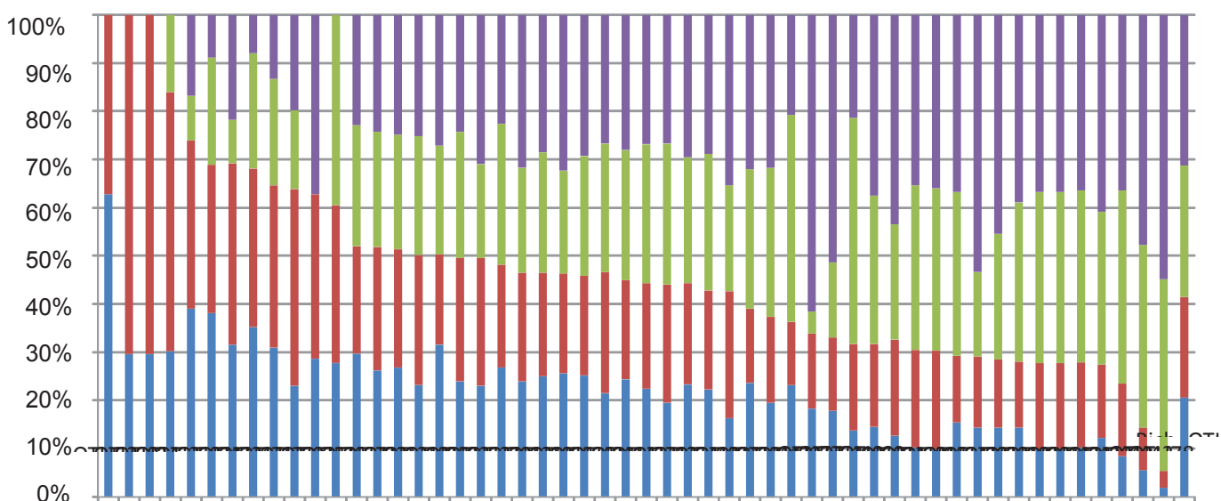
Figure 23: Diagram showing the relative occurrence (presence/absence) of each of the 54 OTUs found in the study for the different modalities (1, 2, 4 and 8 plant species). In blue, red, green and purple are the OTU proportion observed in the 1, 2, 4 and 8 plant species modalities respectively.
