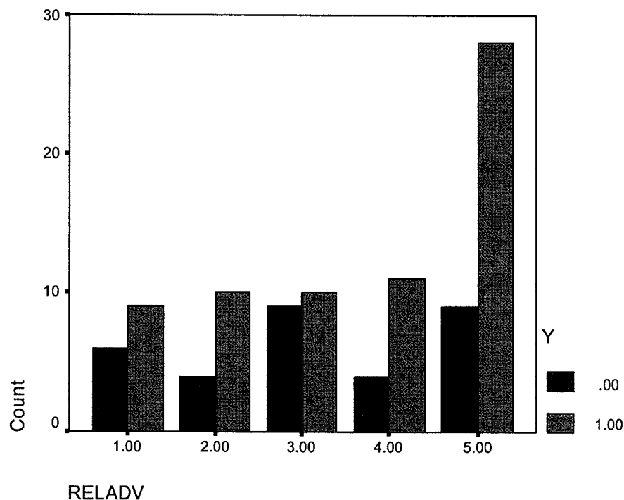
Figure 6.16 – Adopters by variable: reladv
