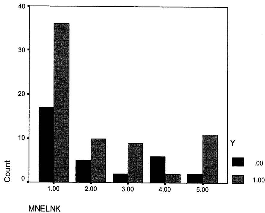
Figure 6.13 – Adopters by variable: mnelnk
