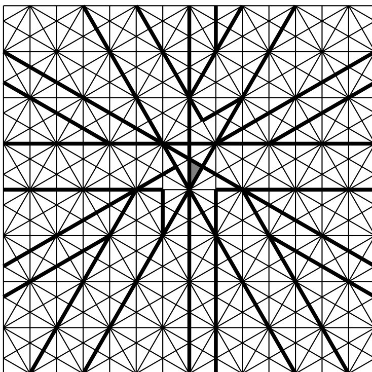
FIGURE 3. r > 2
