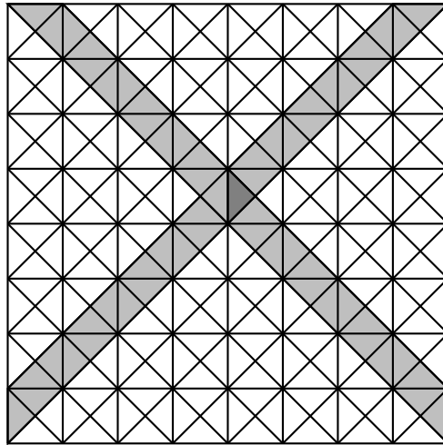
FIGURE 4. Strips of direction \bar{s}_1 containing A_0 .
