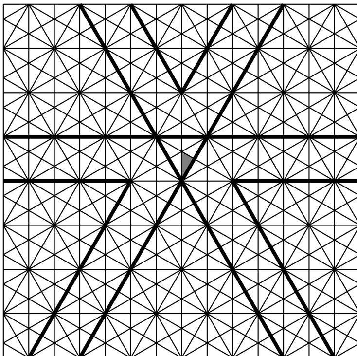
FIGURE 2. r = \infty
