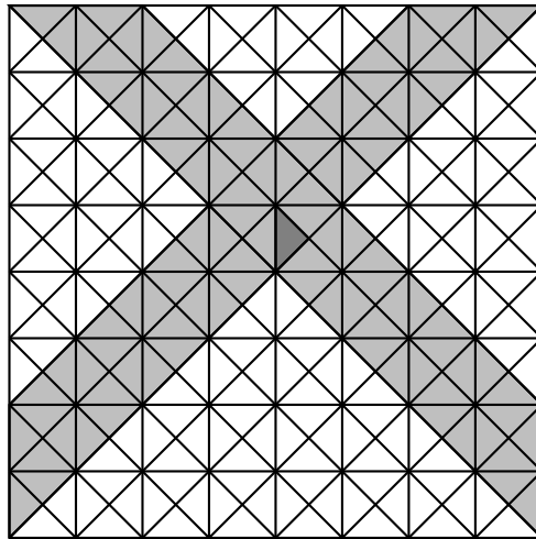
FIGURE 5. Maximal strips of direction \bar{s}_1 containing A_0 .
