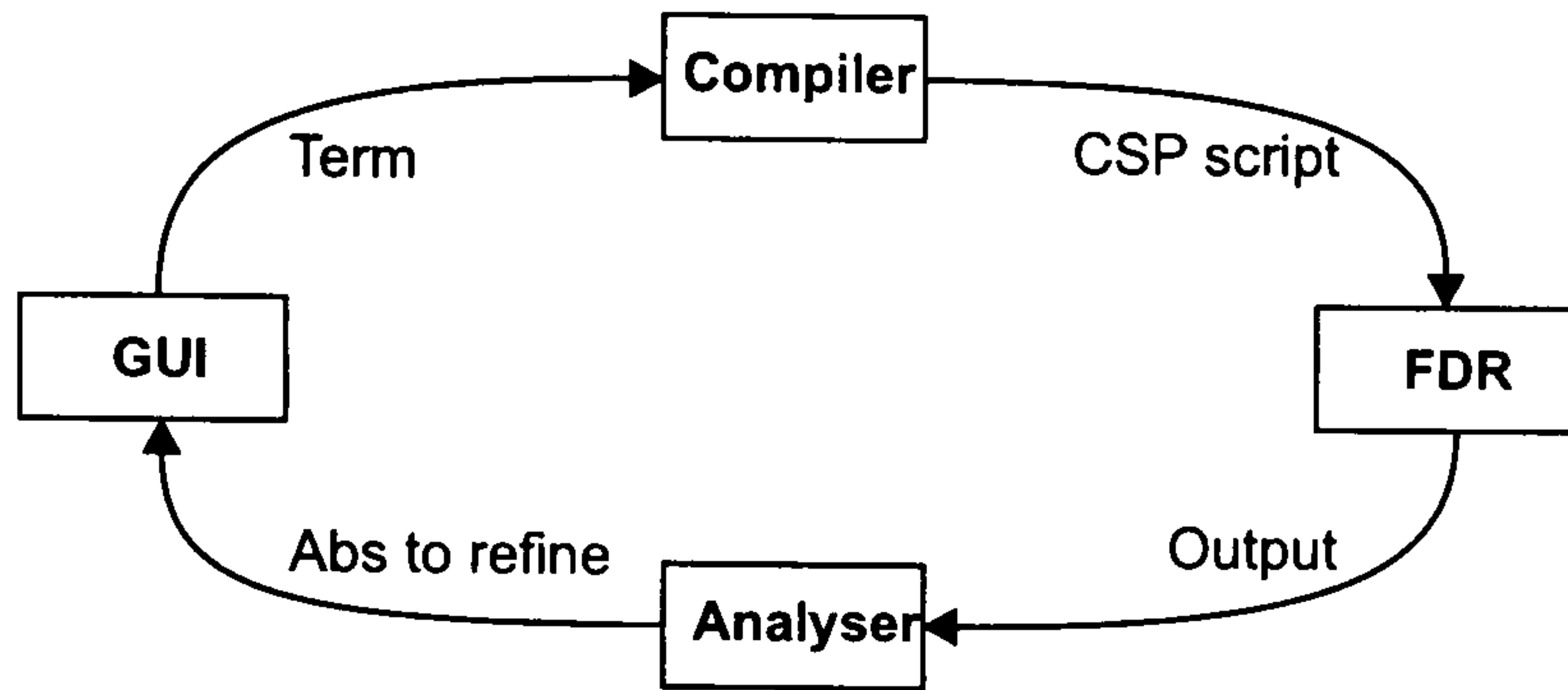
Figure 5.5: The tool architecture
