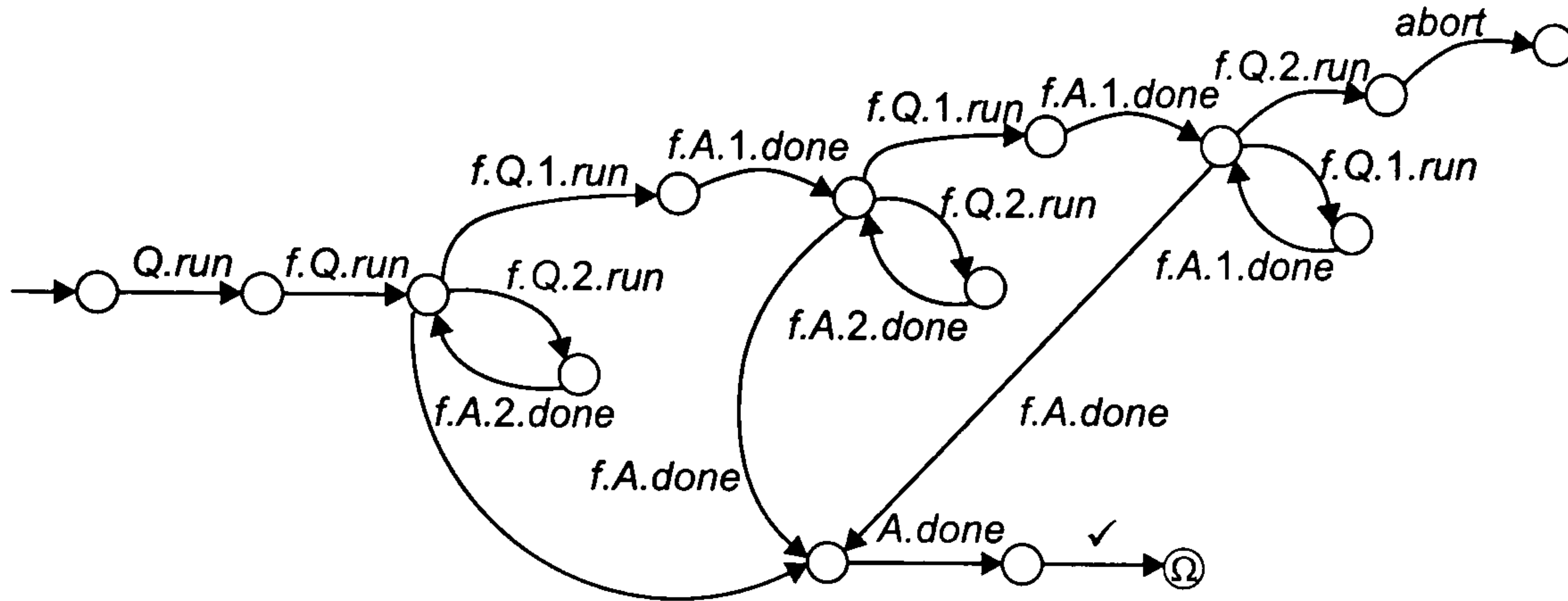
Figure 4.3: A strategy as a labelled transition system
