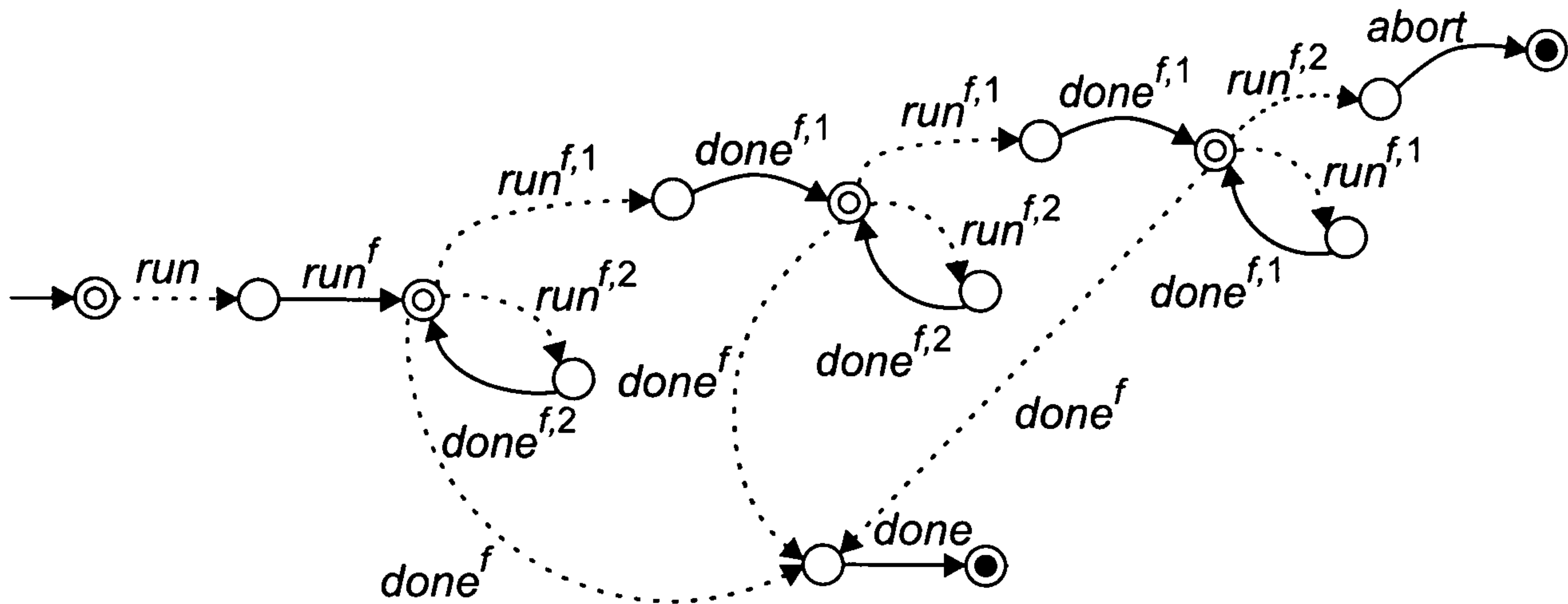
Figure 4.1: A strategy as a finite automaton
