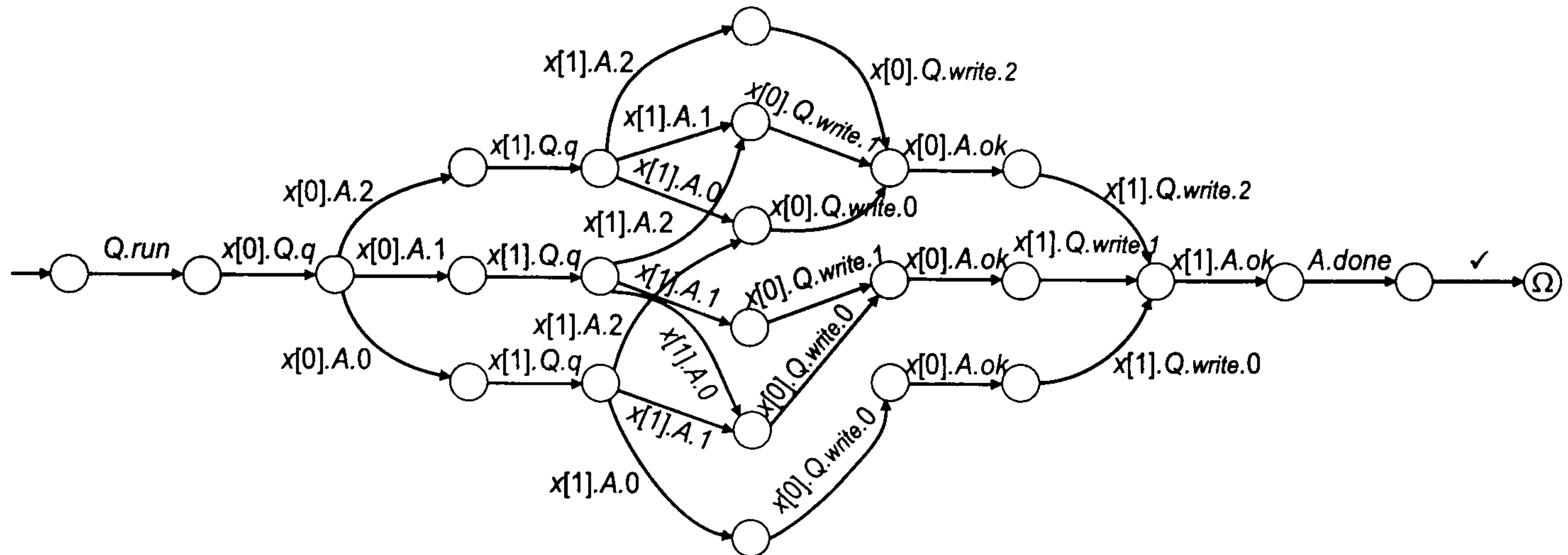
Figure 4.6: LTS for IA 2 bubble sort with k = 2
