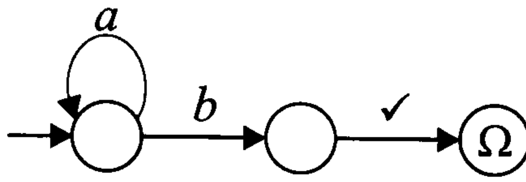
Figure 4.2: A labelled transition system
