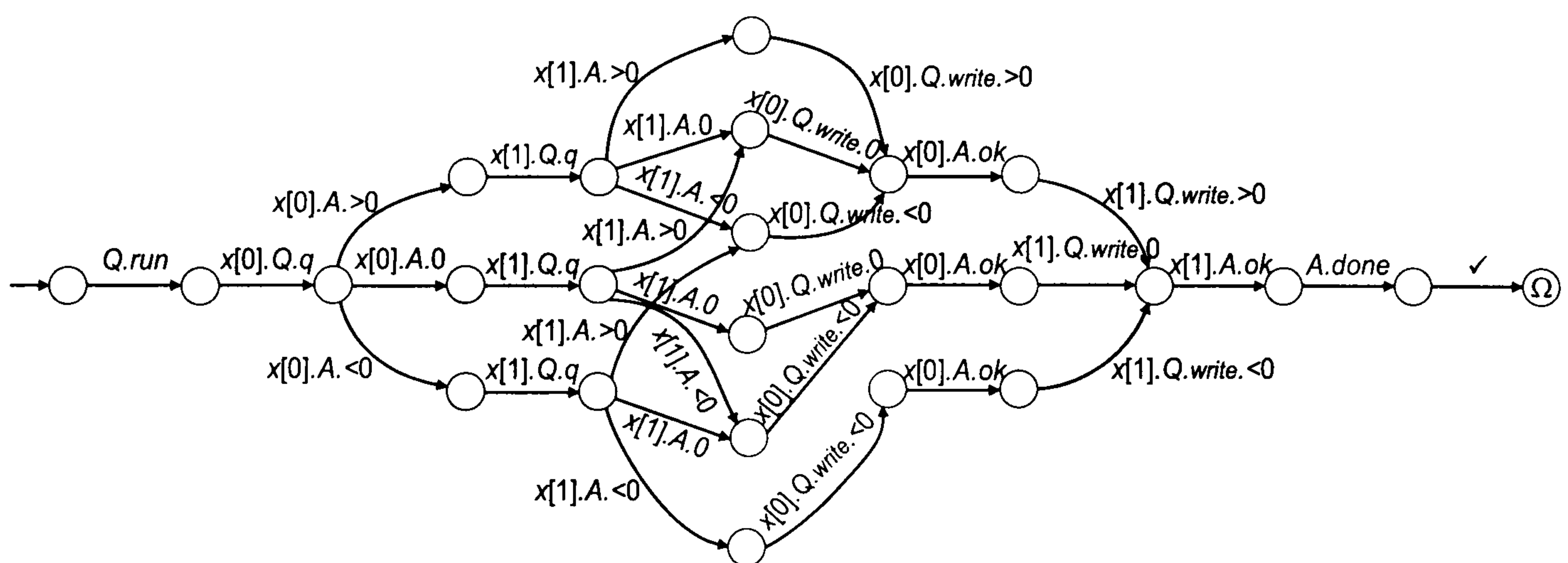
Figure 4.5: LTS for AIA 2 bubble sort with k = 2
