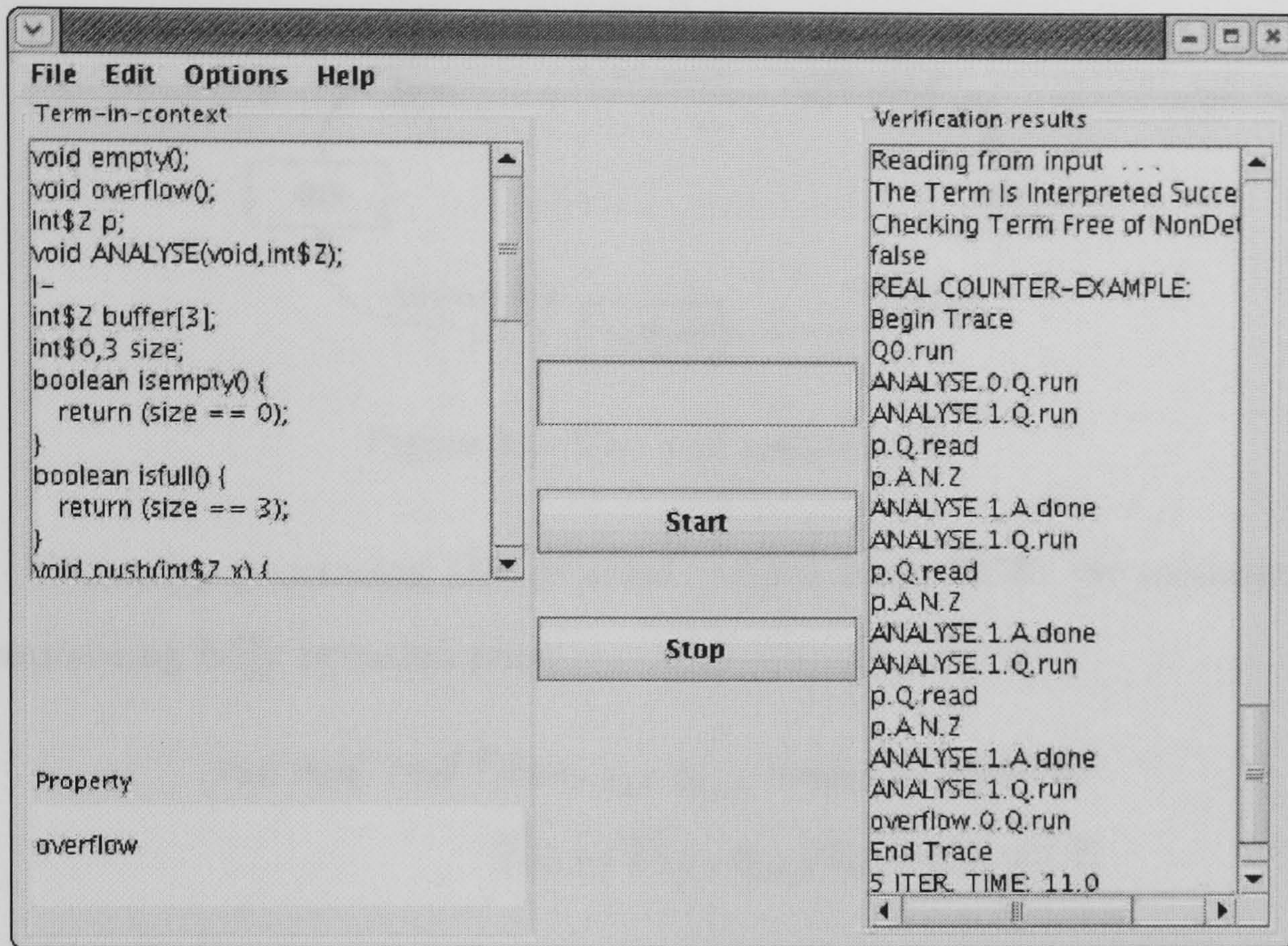
Figure 5.4: A screen-shot of the tool
