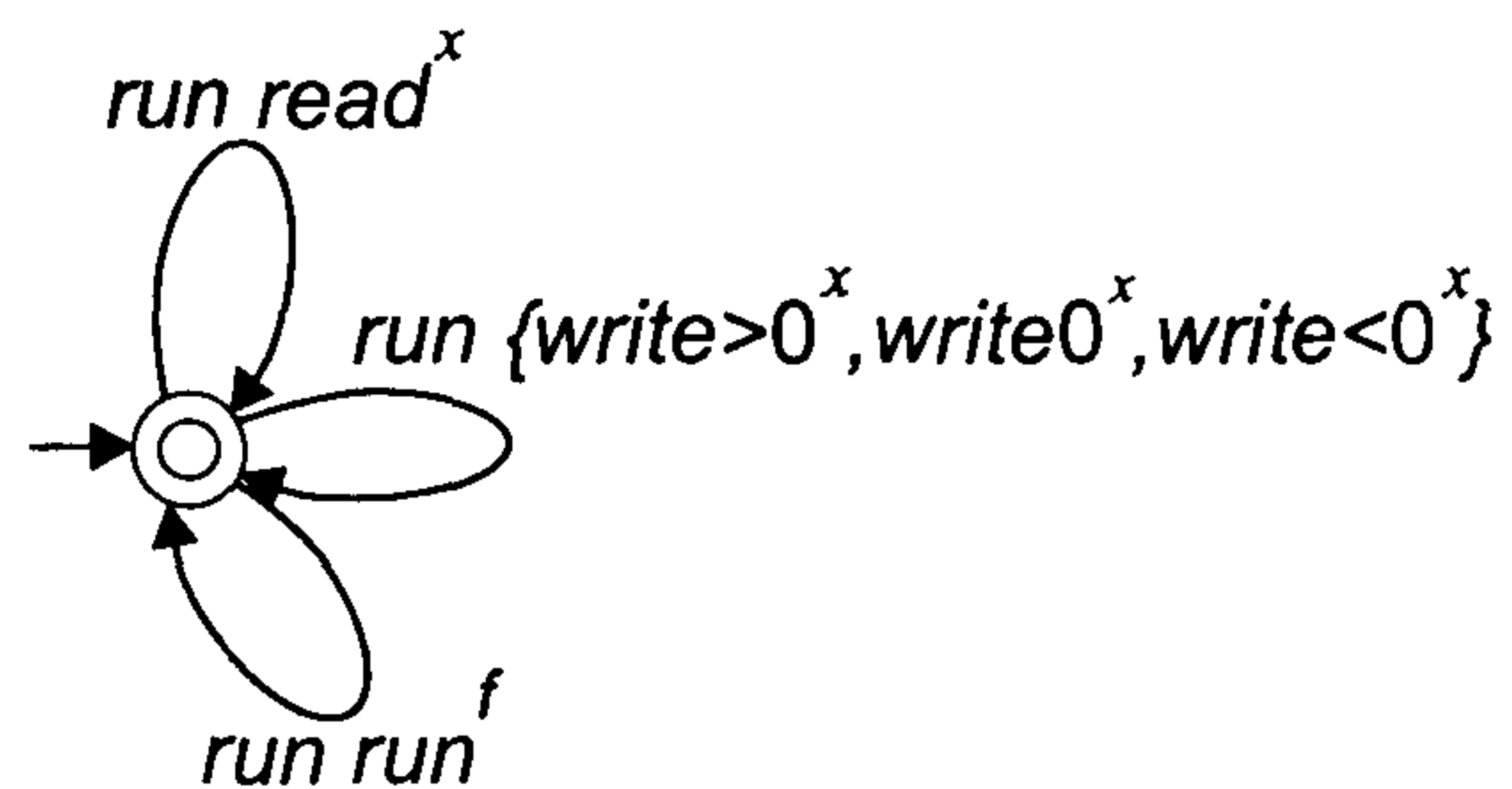
Figure 6.7: Assumption at AR iteration 1
