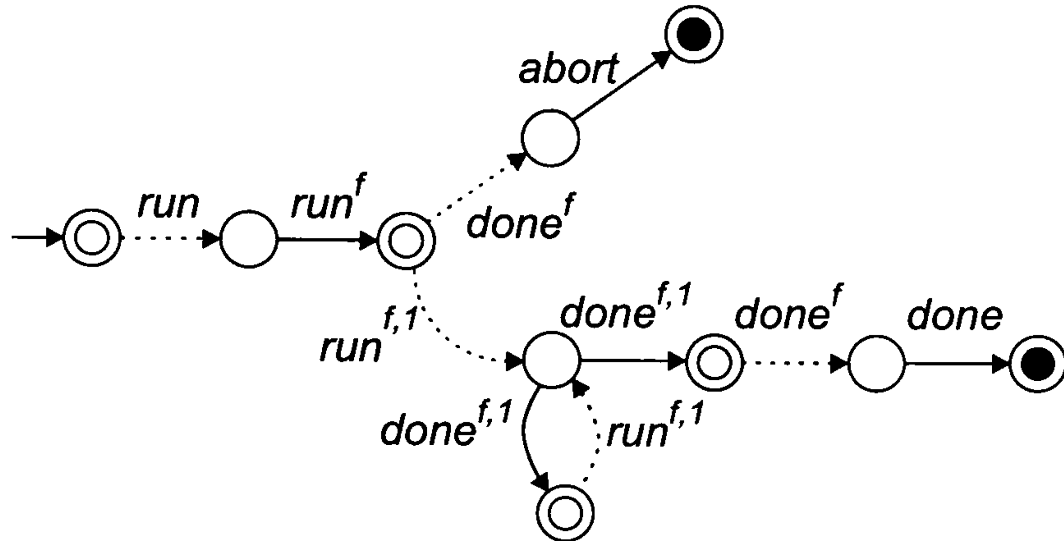
Figure 6.3: The strategy for the running example
