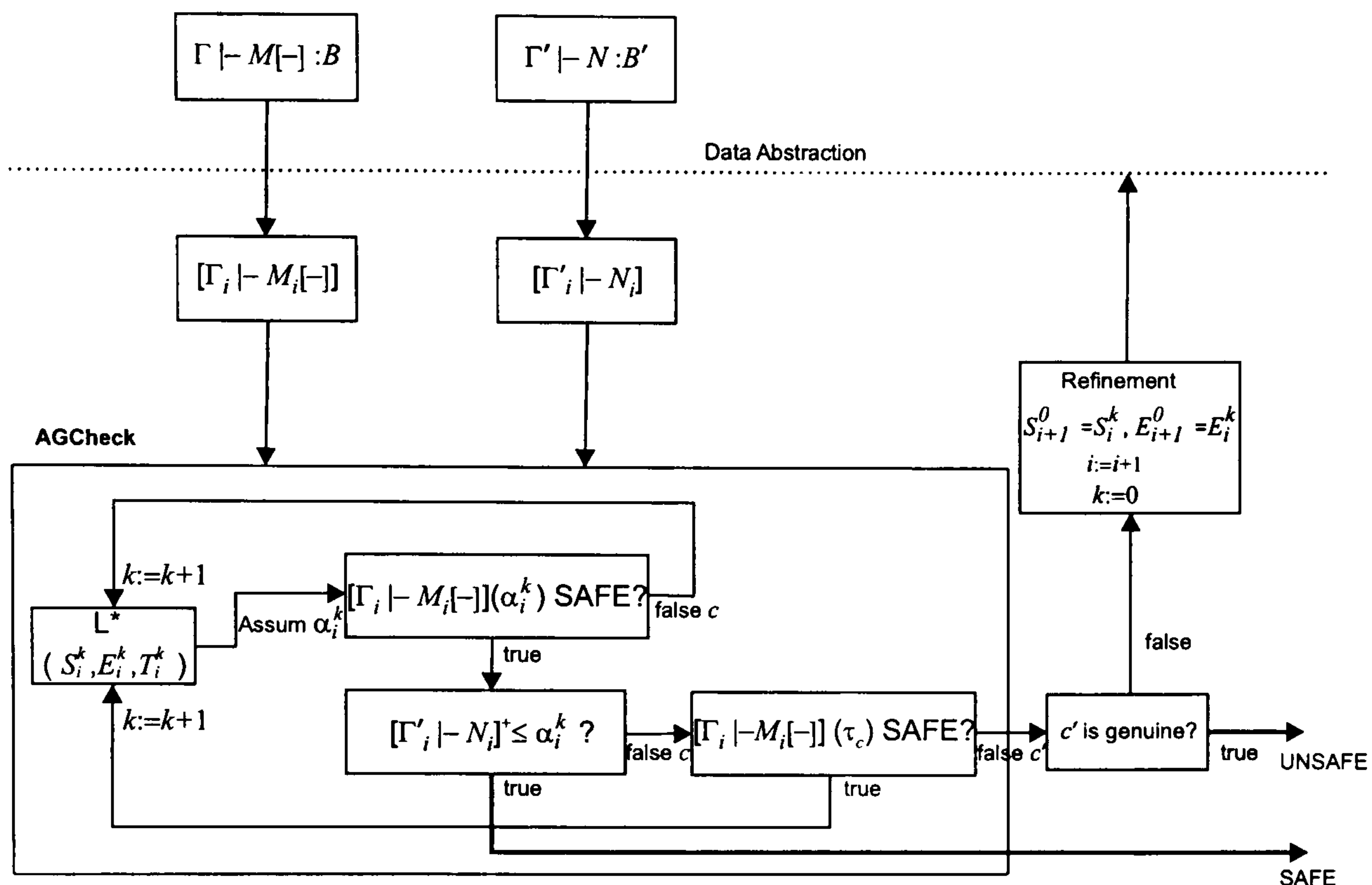
Figure 6.2: Compositional verification procedure
