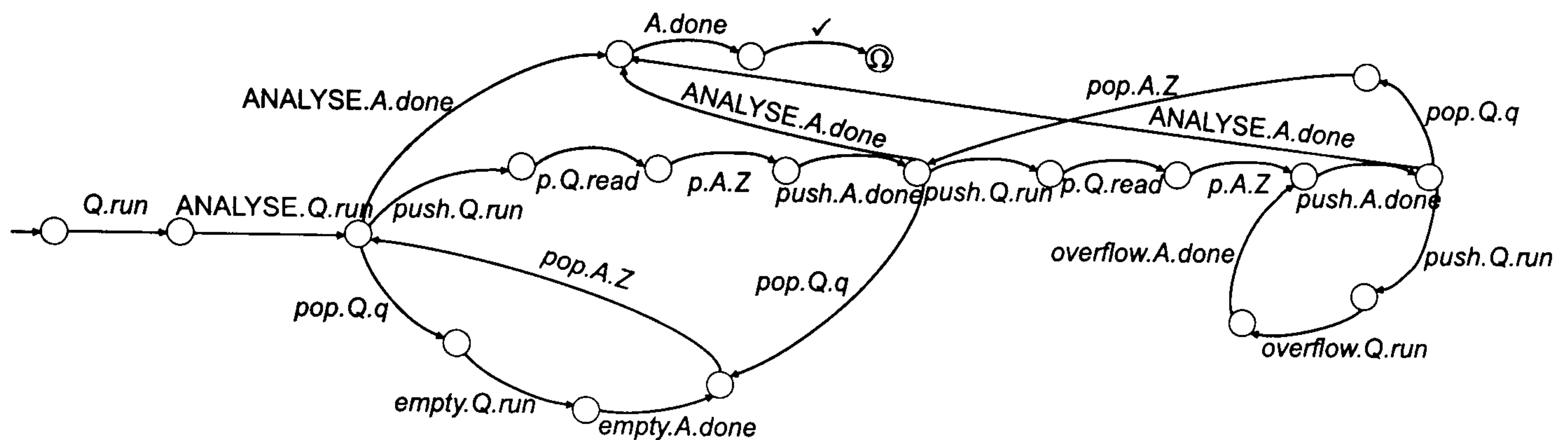
Figure 4.9: LTS for the stack with k = 2
