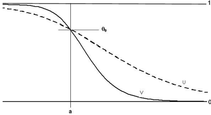
Figure 3.8: \theta_0 in (0, 1) .
