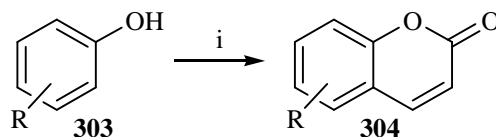
Scheme 4.3. Pechmann condensation in the presence \text{BiCl}_3 . i. Ethyl acetoacetate (1.0 equiv.), \text{BiCl}_3 (5 mol%), 75 °C, 1 – 4 h, 66 – 92%.
