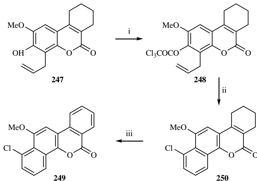
Scheme 3.9. Benzannulation reaction of coumarin 248 . i. \text{Cl}_3\text{CCOCl} , \text{py} , \text{CH}_2\text{Cl}_2 , 0^\circ\text{C} , 62%. ii. \text{CuCl} (5 mol%), ligand 18 (5 mol%), DCE, 200^\circ\text{C} , MW, 2 h, 92%. iii. 10% \text{Pd-C} , \text{Ph}_2\text{O} , 259^\circ\text{C} , \text{N}_2 , 48 h, then in air 24 h, 62%.
