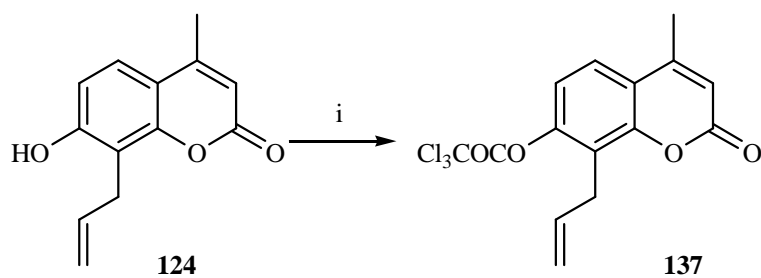
Scheme 2.20. Acylation of coumarin 124 . i. \text{Cl}_3\text{COCOCl} (1.2 equiv.), py (1.2 equiv.), \text{CH}_2\text{Cl}_2 , rt, 16 h, 75% (crude yield).
