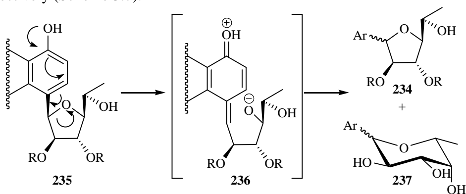
Scheme 3.7. Possible anomerisation of the furanoside.
