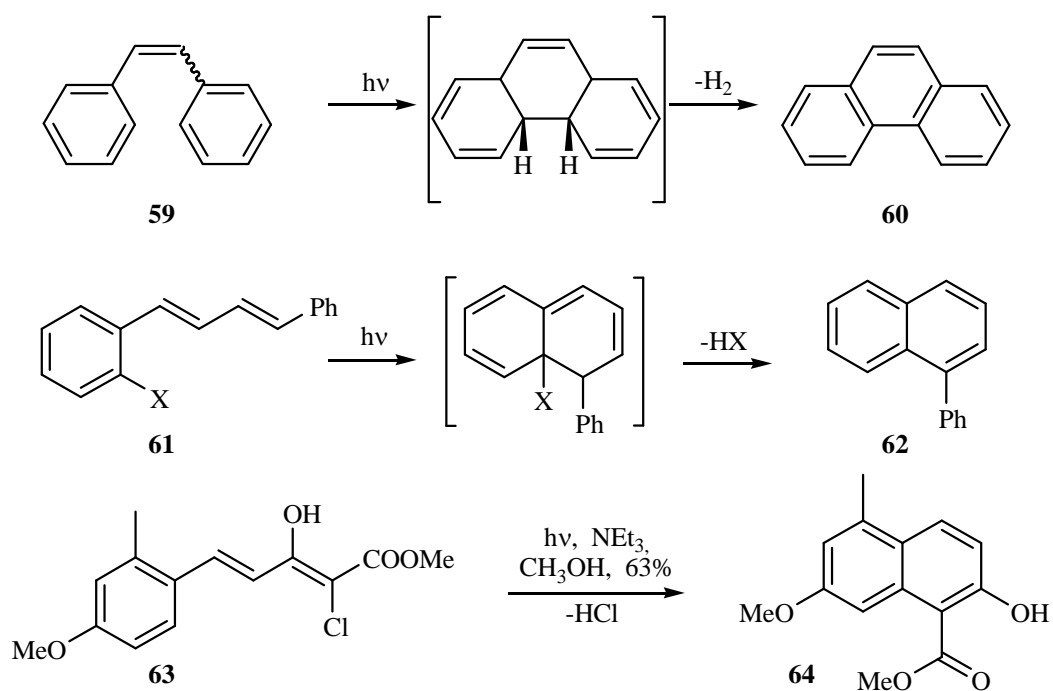
Scheme 1.16. Stilbene photocyclisation
