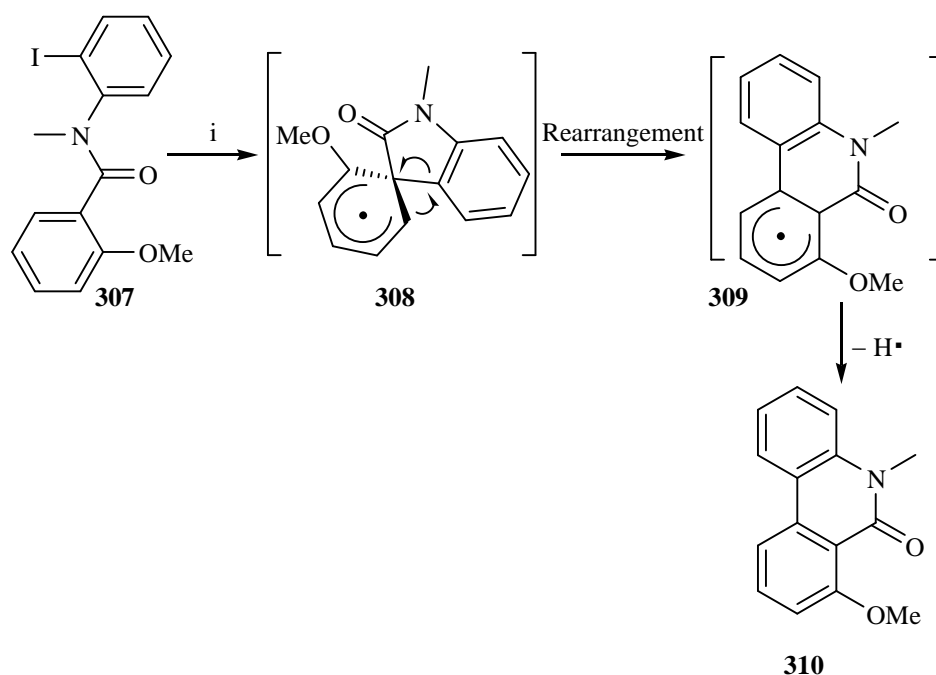
Scheme 4.5. Synthesis of quinolines via rearrangement of spirocyclohexadienyl radicals. i. \text{SmI}_2 (5.0 equiv.), HMPA (18 equiv.), THF, 0 °C, 89%.
