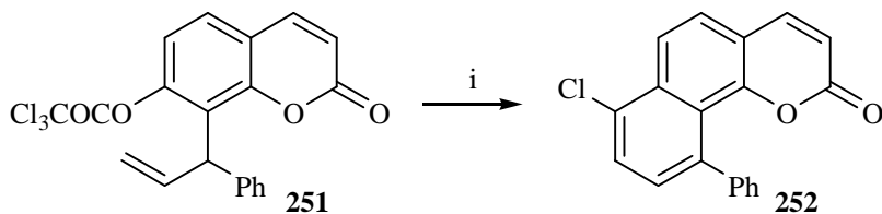
Scheme 3.10. BHQ reaction of sterically congested trichloroacetate 251 . i. \text{CuCl} (5 mol%), ligand 18 (5 mol%), DCE, 200^\circ\text{C} , 2 h, MW, 62%.
