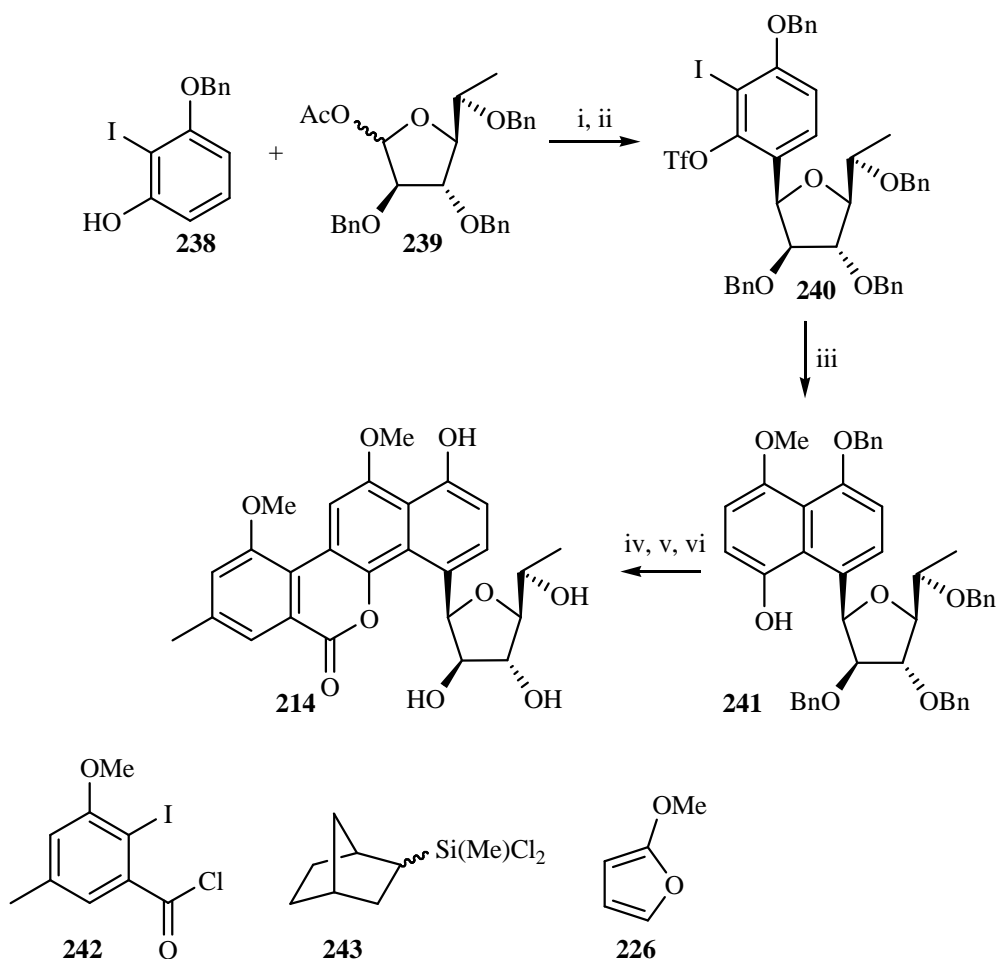
Scheme 3.8. Synthesis of gilvocarcin M. i. 243 -AgClO 4 , CH 2 Cl 2 (-78 to -20 °C), 91%. ii. Tf 2 O, i Pr 2 NEt/CH 2 Cl 2 , -78 °C, 1 h, 99%. iii. n BuLi, 226 /THF, -78 °C, 10 min, 88%. iv. 242 , i -Pr 2 NEt, DMAP (cat.), THF, rt, 2 h, 91%. v. (Ph 3 P) 2 PdCl 2 (26 mol%), NaOAc/DMA, 125 °C, 5 h, 90%. vi. H 2 , 10% Pd-C/MeOH-THF, rt, 5 h, 90%.
