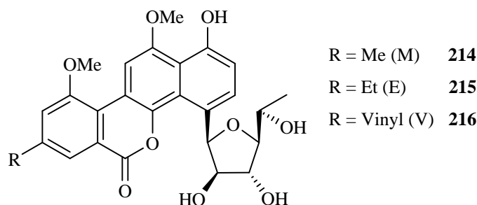
Figure 3.3. gilvocarcin structure.
