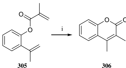
Scheme 4.4. Ring closing metathesis for the formation of coumarin 306 . i. Grubbs' 2 (5 mol%), toluene, 80 °C, 12 h, 45%.
