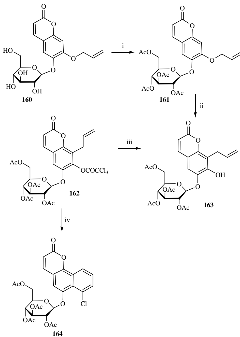
Scheme 2.31. Study of the benzannulation reaction of the esculin derivative 160 . i. \text{Ac}_2\text{O} (11.2 equiv.), py, rt, 17 h, 54%. ii. 210 - 220\text{ }^\circ\text{C} , 5 h. iii. \text{ClCOCCl}_3 (1.2 equiv.), \text{Et}_3\text{N} (1.2 equiv.), \text{Et}_2\text{O} , 0\text{ }^\circ\text{C} , 3 h, 60%. iv. (\text{IPr})\text{CuCl} ( 156 , 5 mol%), DCE, 200\text{ }^\circ\text{C} , 2 h, MW, 21%.
