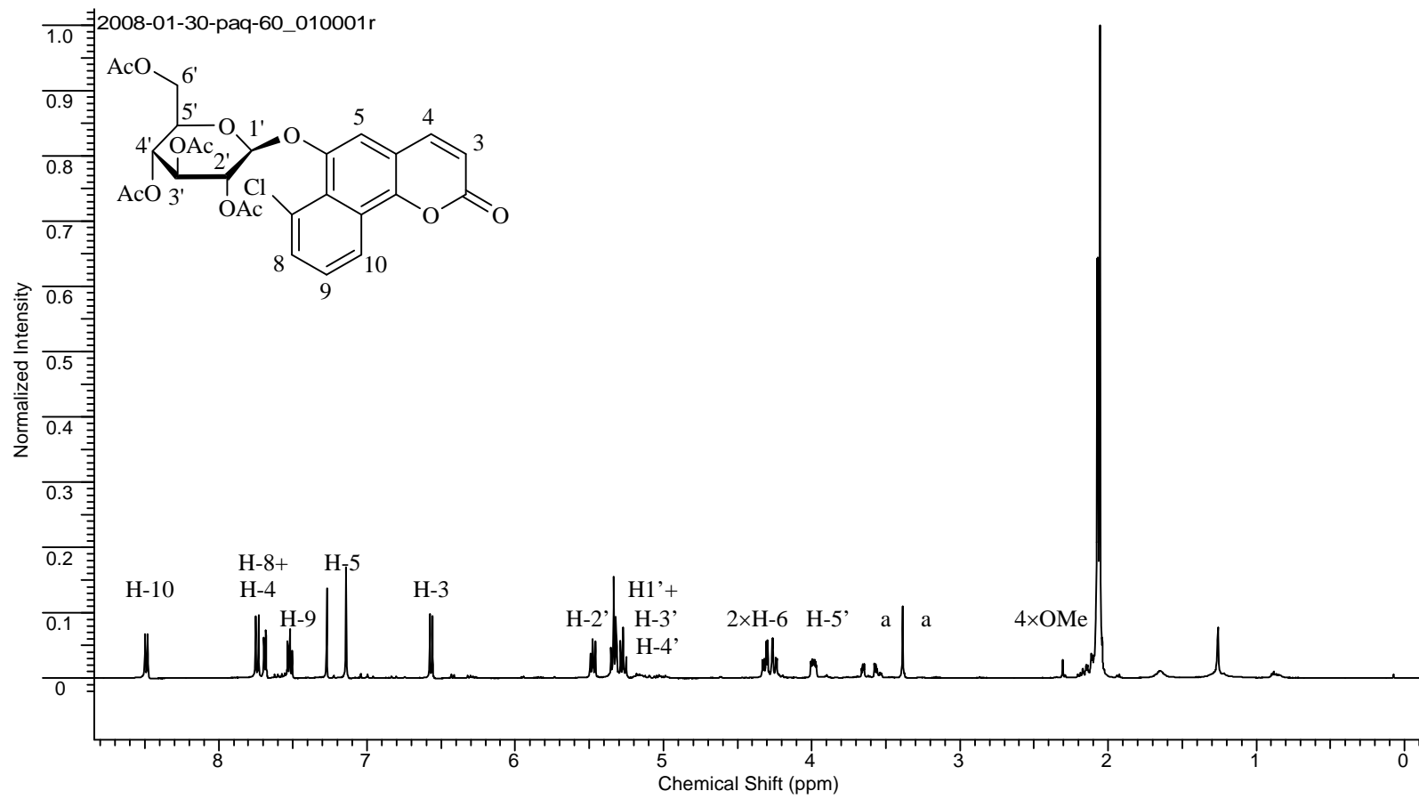
Figure 2.6. ^1\text{H} NMR of glycoside 162 . a. Peaks due to diglyme.
