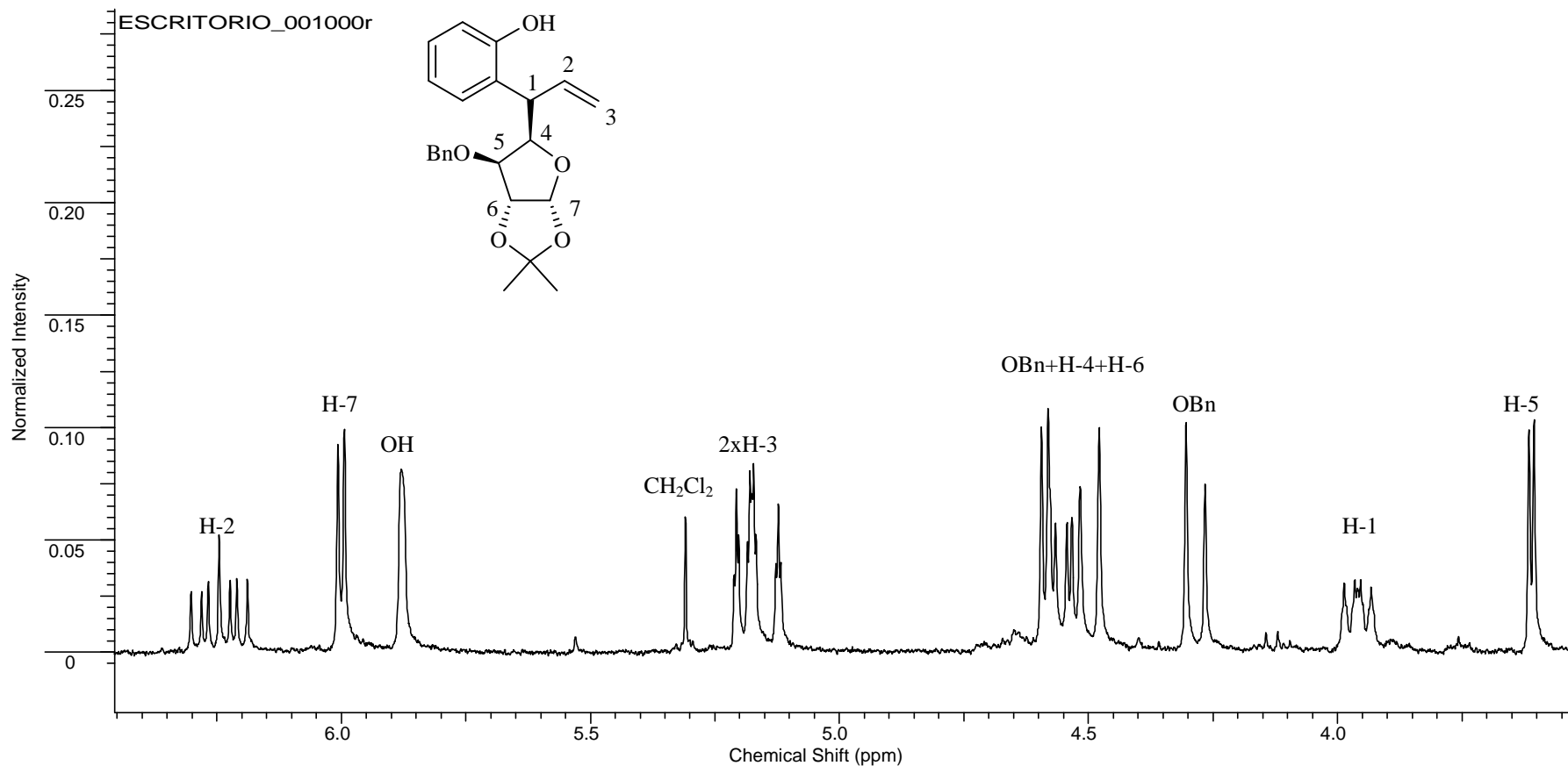
Figure 3.12. Characteristic peaks of the carbohydrate allyl phenol 272 ^1\text{H NMR} ( \text{CDCl}_3 ).
