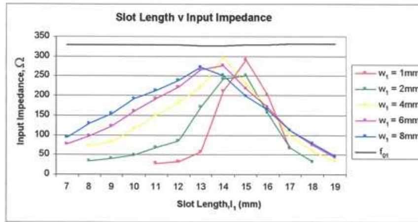
\epsilon_r = 2.33, h = 1.57 \text{ mm}, L = W = 30 \text{ mm}, s_1 = 1 \text{ mm} (b)
