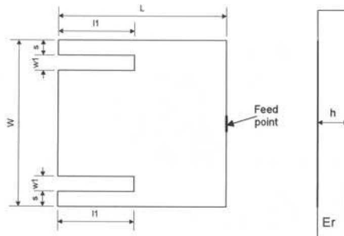
Figure 7.15: Patch design A
