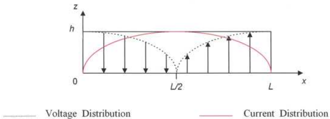
Figure 5.12 Field configuration of TM_{01} mode
