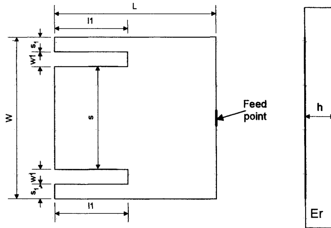
Figure 7.10: Compact patch configuration - Design A
