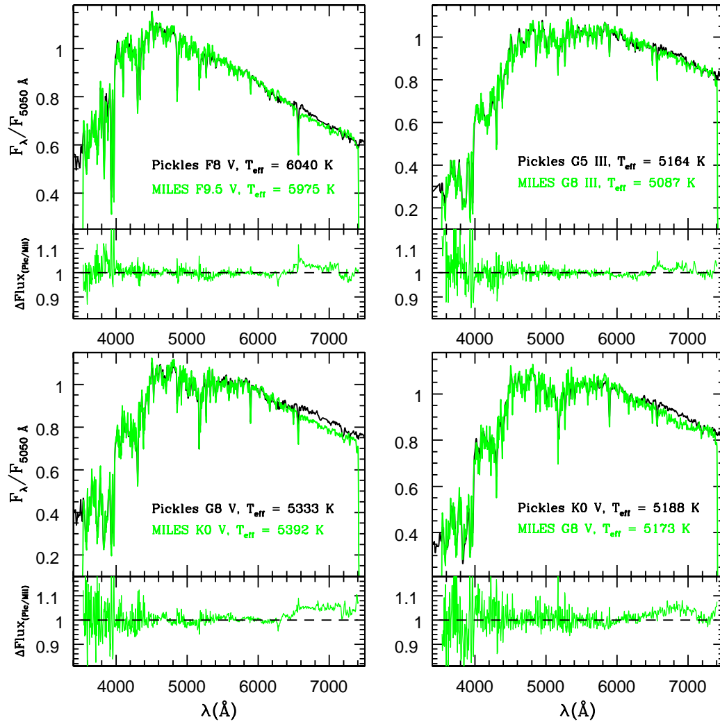
Figure 5.17: Best-fitting MILES spectra to four standard Pickles spectra, accompanied by their respective flux ratios as a function of wavelength, defined as \Delta F_\lambda = F_{\lambda, \text{Pickles}} / F_{\lambda, \text{MILES}} (smaller panels). Flux ratios are scattered around 1, except between 6500 and 7000 \text{\AA} , where a systematic flux deficiency in the MILES spectra can be observed. For this exercise the MILES spectra have been smoothed and rebinned to the Pickles resolution and sampling.
