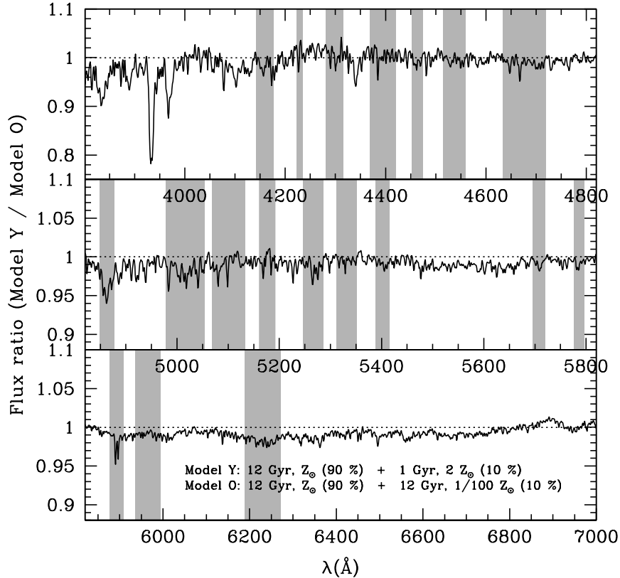
Figure 6.3: Flux ratios between Models Y and O, normalised around 5050 Å for a 10% minor component. Shaded areas represent the common Lick/IDS index passbands as defined by Trager et al. (1998) ( \text{CN}_2 and \text{Mg}_2 have been omitted, since they overlap with \text{CN}_1 and \text{Mgb} , respectively). Notice the large difference in Ca K strength at 3933.7 Å.
