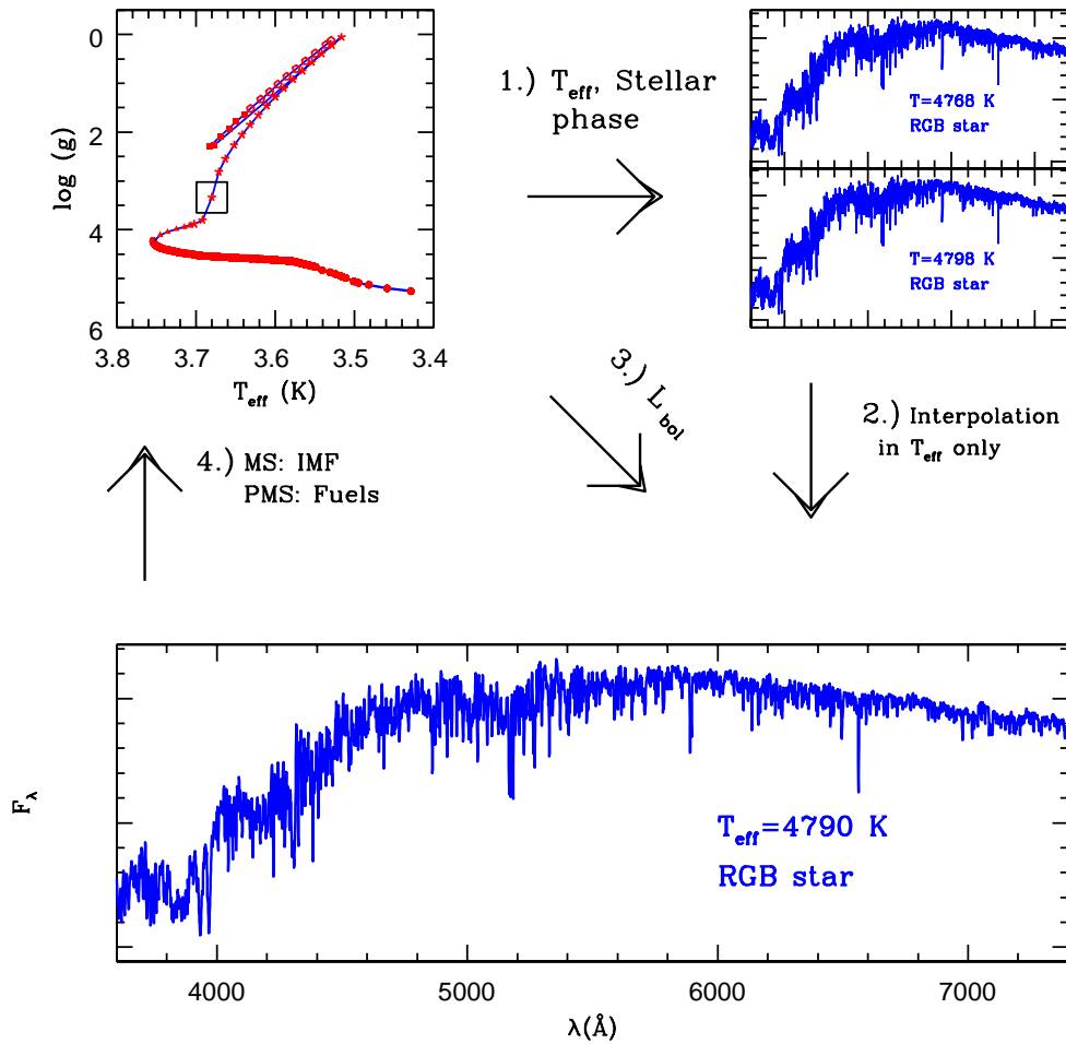
Figure 2.4: Same as Fig.2.2, but for empirical stellar spectra. The symbols in the upper left panel denotes respectively: filled circles =MS, filled triangles =SGB, stars =RGB, filled squares =HB, and open pentagons =E-AGB.
