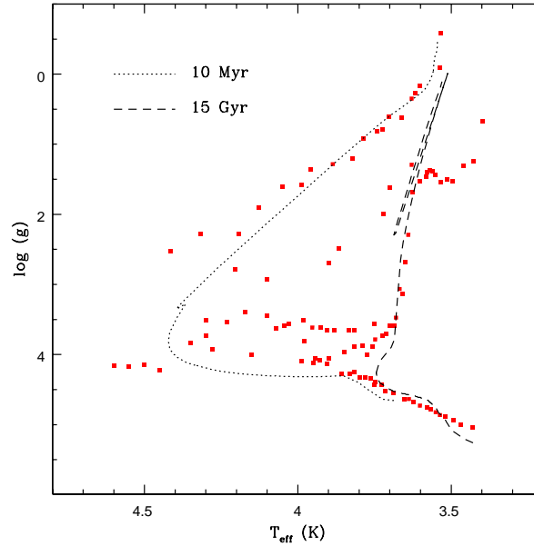
Figure 3.2: Evolutionary coverage at Z_{\odot} for the Pickles library. Superimposed are the 10 Myr and 15 Gyr isochrones (MS) and stellar tracks (PMS) that are used in the synthesis (see M05 for a description of the isochrones and tracks).
