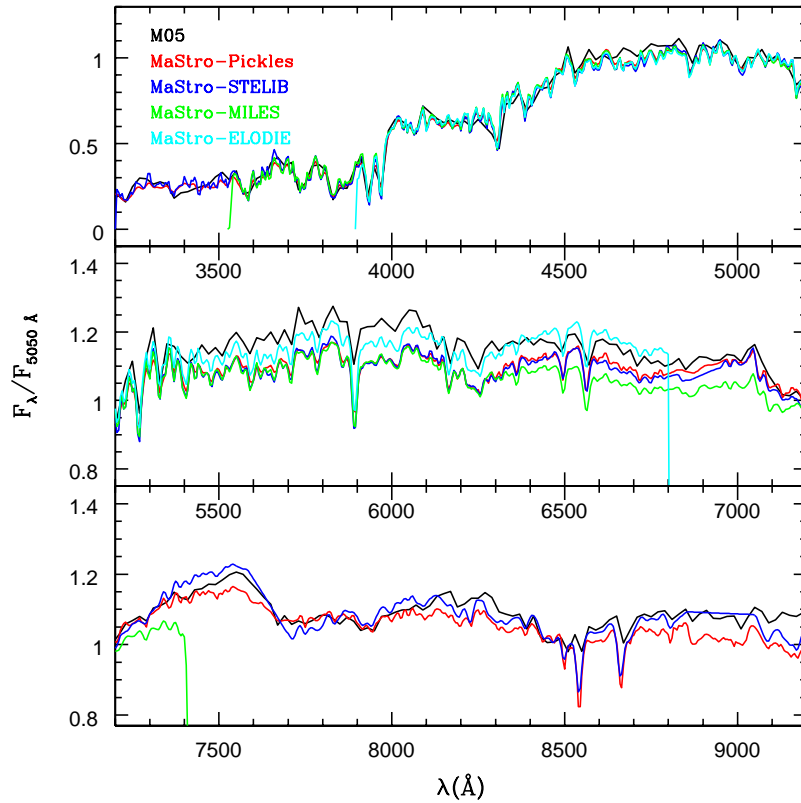
Figure 4.9: Same as Fig.4.8, but for a 12 Myr, Z_{\odot} SSP with Salpeter IMF. Notice the considerable drop in flux between 5500 and 7000 \text{\AA} for a majority of the models based on empirical libraries compared to the M05 model.
