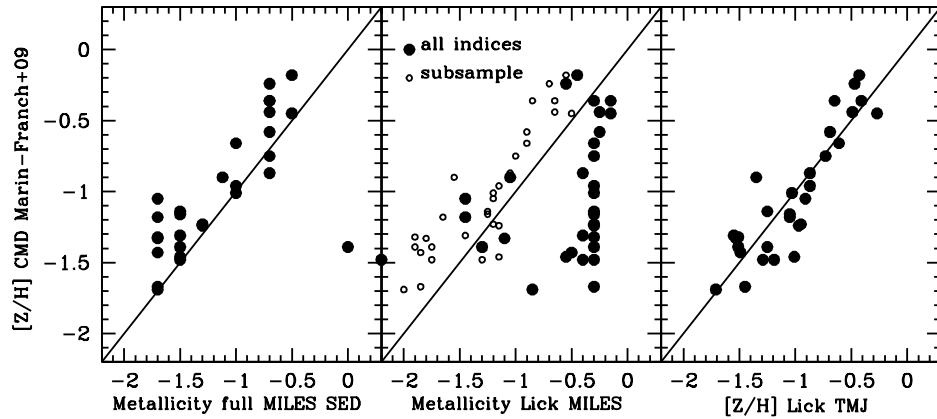
Figure 5.5: Same as in Fig.5.3, but for the CMD-derived metallicities of Marín-Franch et al. (2009) instead, which are corrected for abundance ratio effects and therefore considered to reflect total metallicity.
