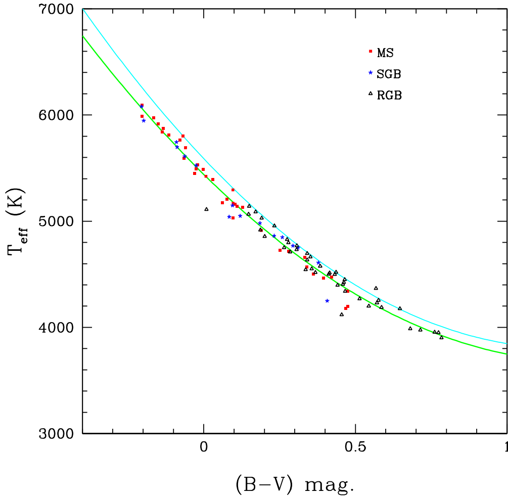
Figure 4.15: (B-V) colour-temperature relation for solar metallicity MILES stars ( green ) in the temperature range important for turnoff and RGB bump stars in old stellar populations. Overplotted is the same relation for STELIB stars ( cyan ). All data points are MILES stars.
