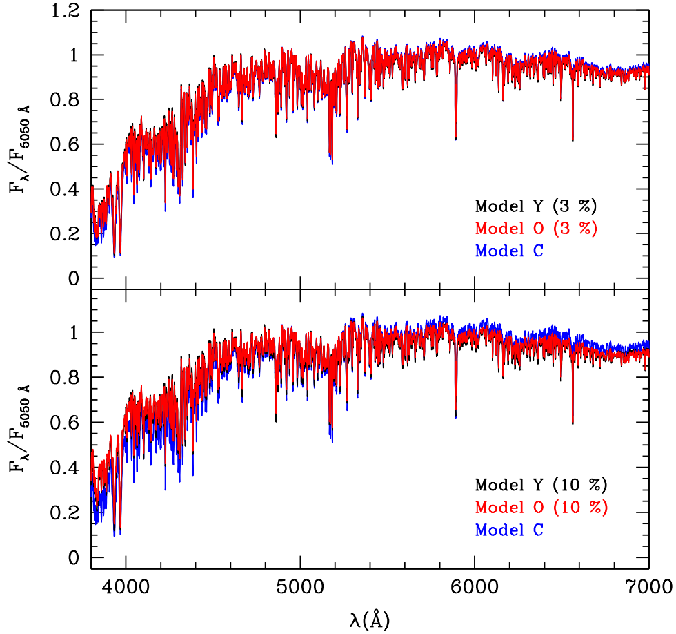
Figure 6.1: Comparison of the SEDs of Models Y, O, and C, normalised around 5050 \text{\AA} , given a minor component fraction of 3 % ( upper panel ) and 10 % ( lower panel ).
