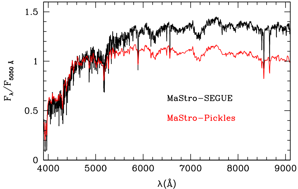
Figure 7.2: Comparison of 12 Gyr, Z_{\odot} MaStro SSPs based on the Pickles and SEGUE libraries ( red and black , respectively). The considerably redder colours of the latter is due to the temperature scale adopted for the SEGUE spectra.
