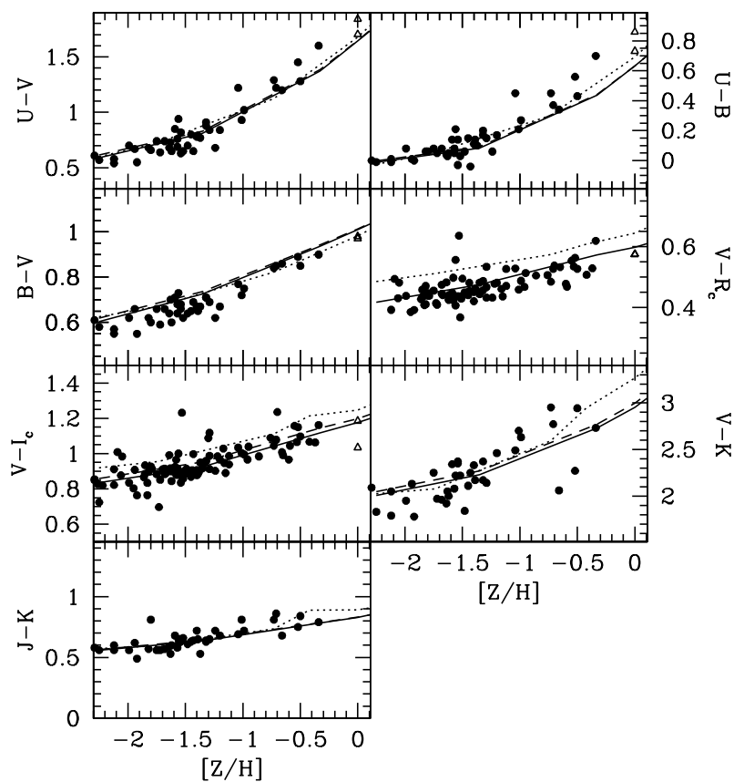
Figure 1.1: Reprint of Fig.21 in Maraston (2005) . The broadband colours of Milky Way globular clusters are plotted as a function of metallicity and compared to the 13 Gyr EPS models of Maraston (2005 , solid and dashed lines for Kroupa and Salpeter IMF, respectively) and Bruzual & Charlot (2003 , dotted line, Kroupa IMF).
