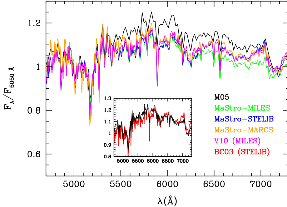
Figure 4.19: The spectral region around the V -band for various 10 Gyr, Z_{\odot} SSP models with Salpeter IMF. All high-resolution models have been smoothed to the resolution of the Pickles library. Apart from the BC03-STELIB model (inset), all empirical MaStro models, as well as the theoretical MaStro-MARCS, and the completely independent V10 model, display the characteristic flux drop around 6000 Å.
