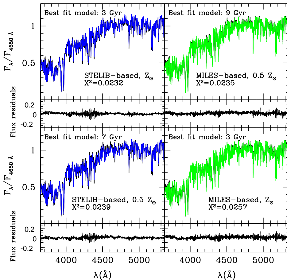
Figure 5.10: First ranked fits at Z_\odot and 0.5 Z_\odot of the MaStro-STELIB ( blue ) and MaStro-MILES ( green ) models to the composite spectrum of Galactic open cluster M67 ( Schiavon et al., 2004 , black ). The residuals to each fit is given below the respective panel.
