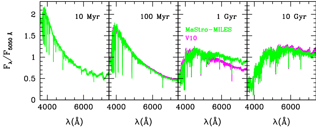
Figure 4.18: Similar to Fig.4.17, but comparing MILES-based MaStro ( green ) and V10 ( magenta ) SSPs, still fixed at Z_{\odot} . No V10 model exists at 10 Myr. The large discrepancy in the 1 Gyr model is due to a lack of proper TP-AGB treatment in the V10 model.
