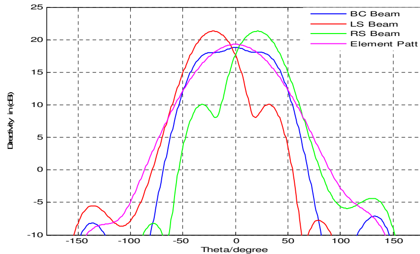
Fig.9.8: Shaped beams @ downlink f_c
