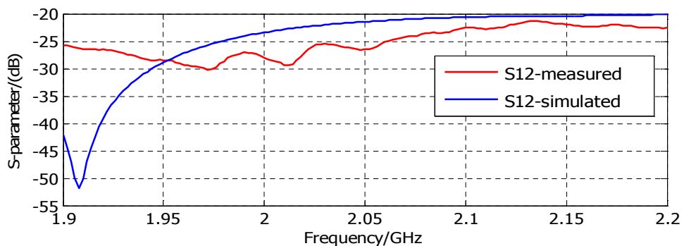
Fig.8.3: Measured and simulated isolation ( S_{12} ) between two ports of single element
