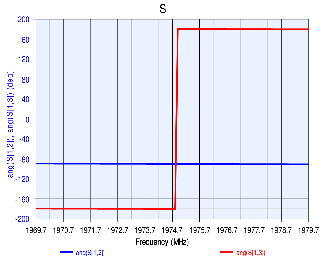
Fig .6.13: Phase different between port2 and 3 ( \arg[S_{12}] - \arg[S_{13}] ) of ideal branch line coupler
