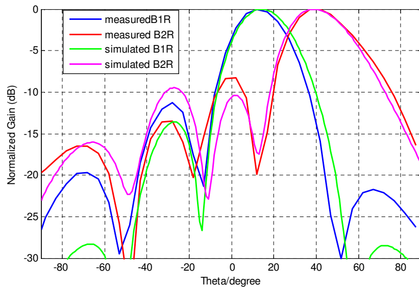
Fig.8.17: Measured and simulated multiple beams @uplink f_c
