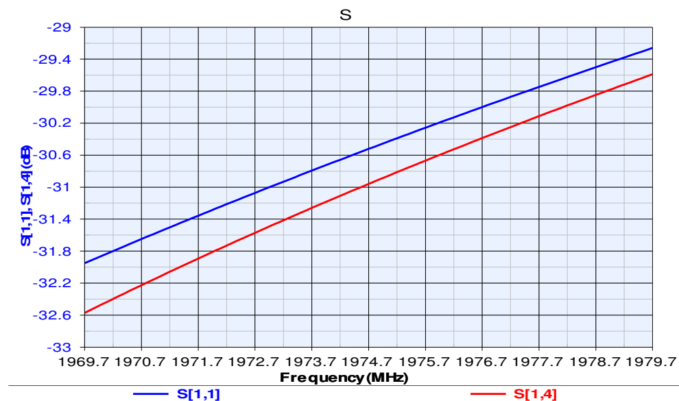
Fig.6.14: Return loss ( -S_{11} dB) and Isolation ( -S_{14} dB) of microstrip branch line coupler
