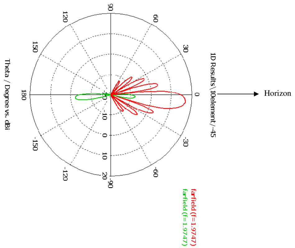
Fig.6.8: Elevation pattern of column array of -45^{\circ} polarisation port
