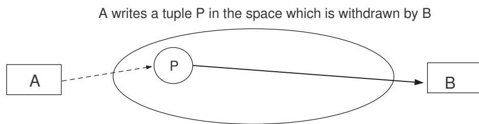
Figure 2.1: Tuple Space
