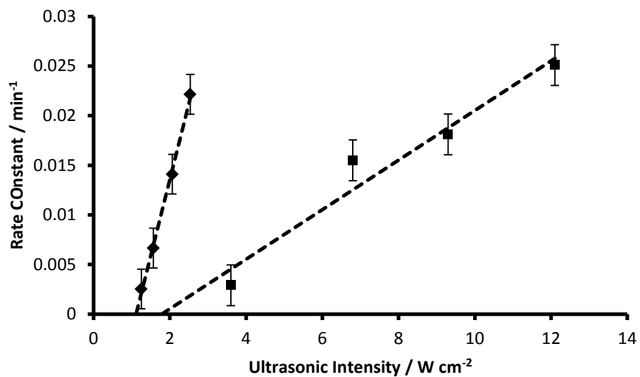
Figure 5.30: Rate constant information for 20 (black squares) and 515 kHz (black diamonds) ultrasound driven degradation experiments
