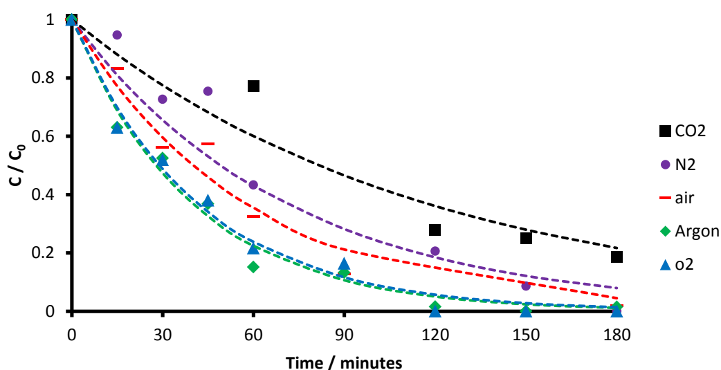
Figure 5.14: Degradations of 100 µg L -1 DBP solutions with different dissolved gas contents. Degradations were performed using 515 kHz ultrasound at an intensity of 2.5 W cm -2 . The temperature was controlled to be 18±2°C.
