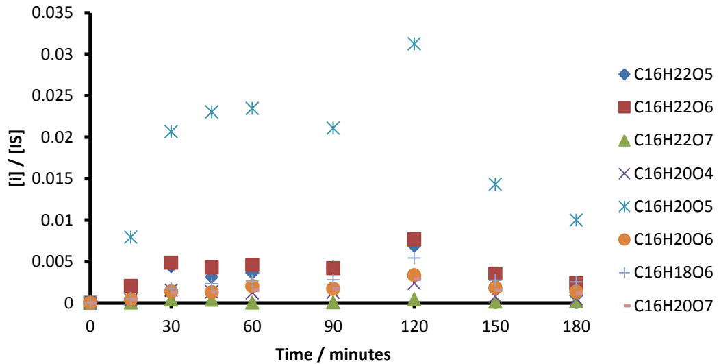
Figure 6.23: Products found via positive mode ionisation of DBP degradation samples (air)
