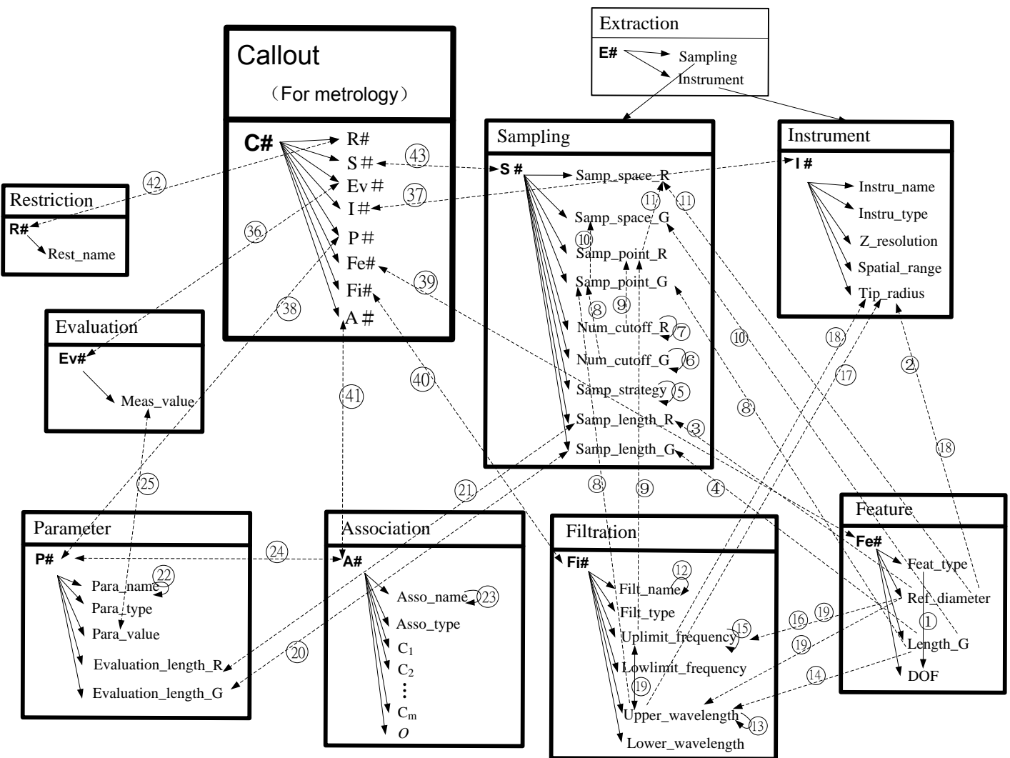
Figure 5.14 The Categorical data model for cylindricity(for Metrology)
