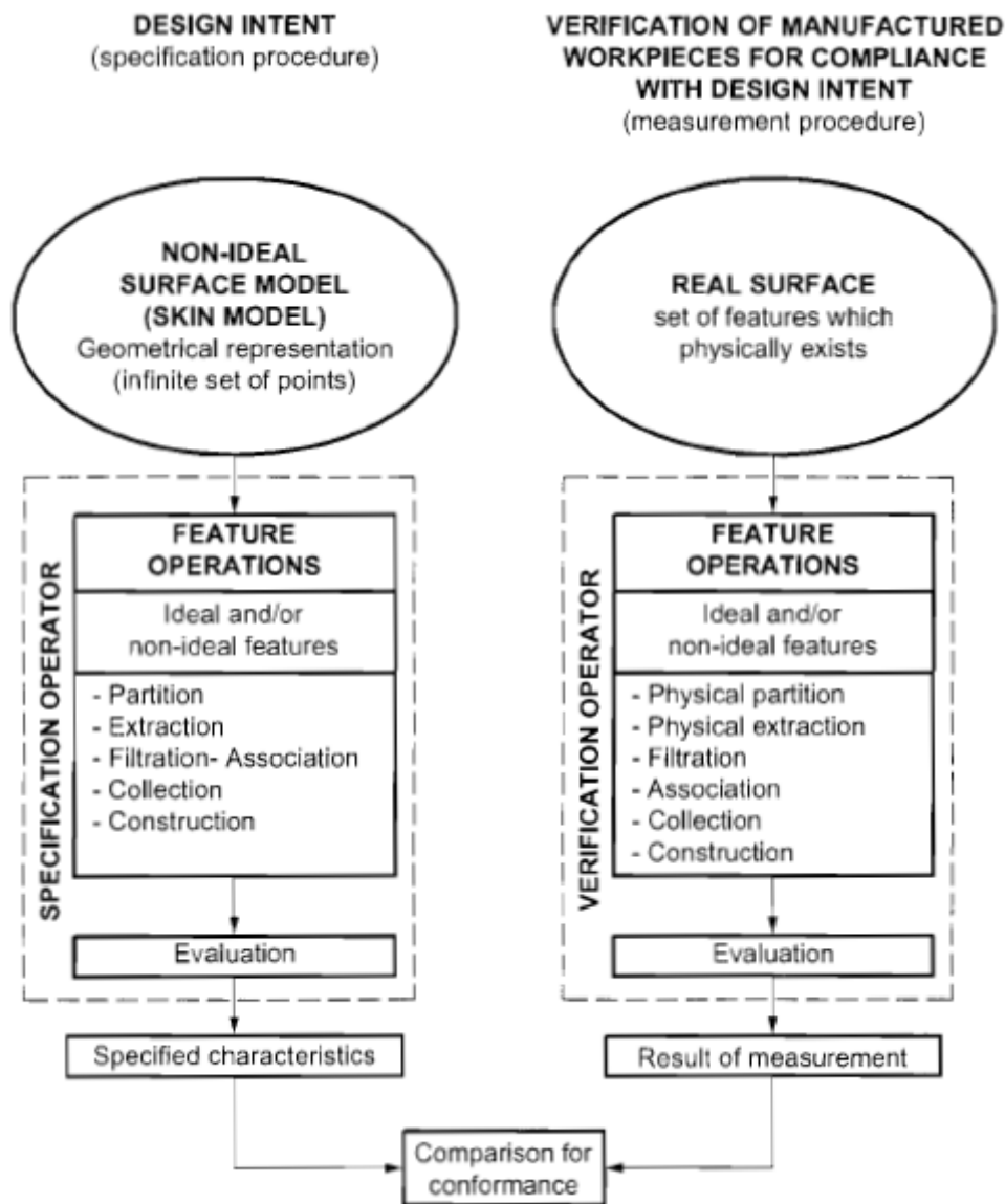
Figure 2.5 Mirror between Specification and Measurement procedures [91]
