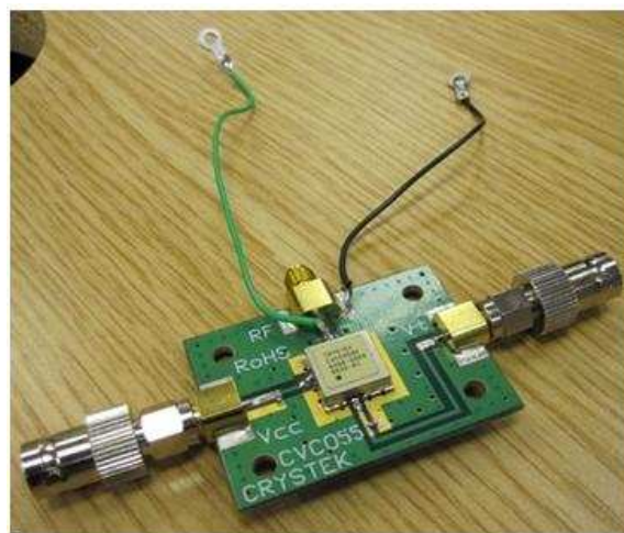
Figure 5-5 (b) CRYSTEK - CVCO55B Voltage Controlled Oscillator
