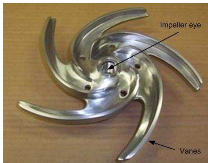
Figure 2-4 Open impeller
