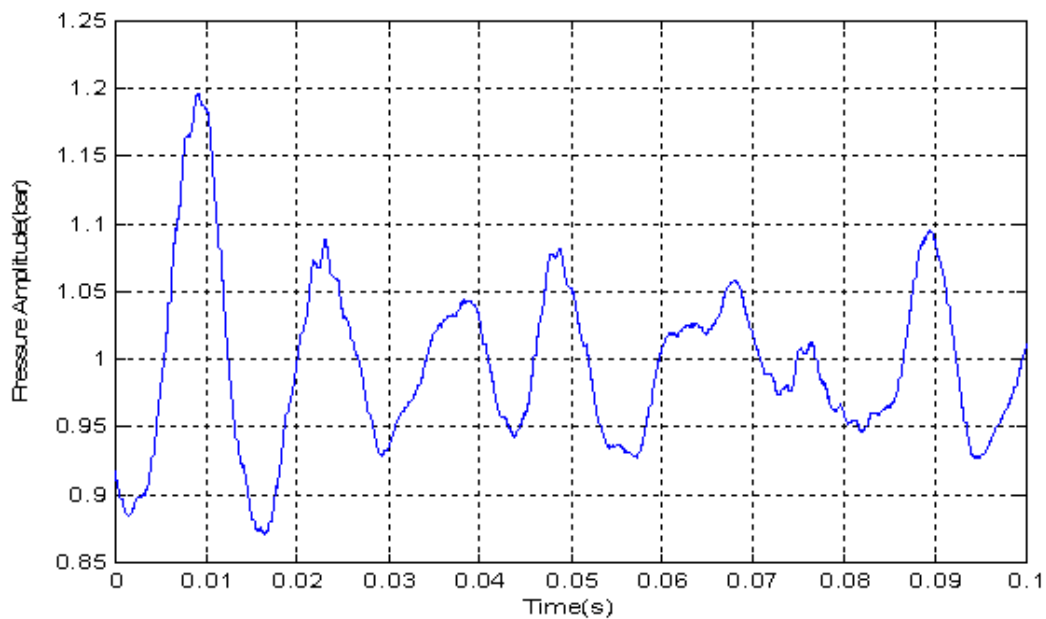
Figure 4-10 Typical online raw data measured by pressure transducer in suction line
