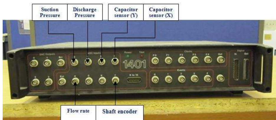
Figure 4-24 CED 1401 Plus data acquisition system
