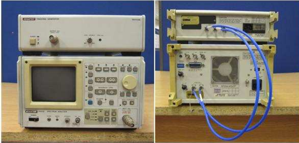
Figure 5-6 Advantest type R4131D spectrum analyser
