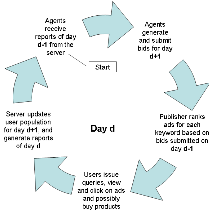
Figure 3.1: Daily activities cycle in TAC AA.
