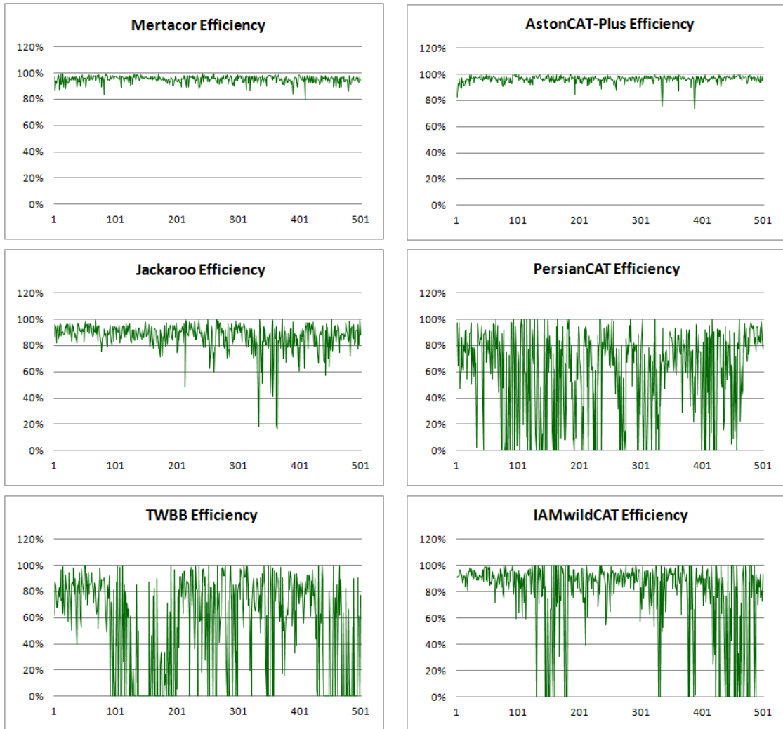
Figure 4.10: Allocative Efficiency of each agent in a typical heterogeneous game.
