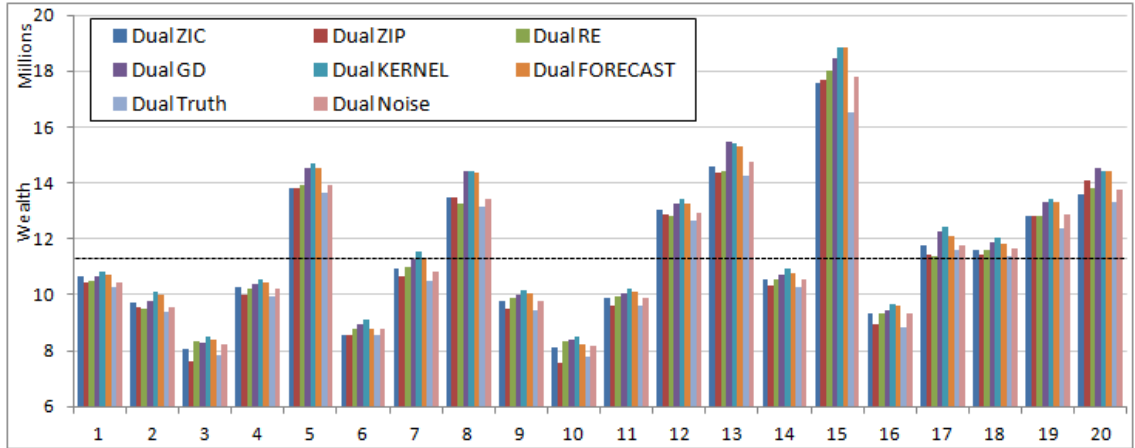
Figure 5.17: Final wealth each trader group possess in dynamic heterogeneous games. From left to right, strategy of the group is Dual ZIC, Dual ZIP, Dual RE, Dual GD, Dual Kernel, Dual Forecast, Dual Truth and Dual Noise (20 iterations).
