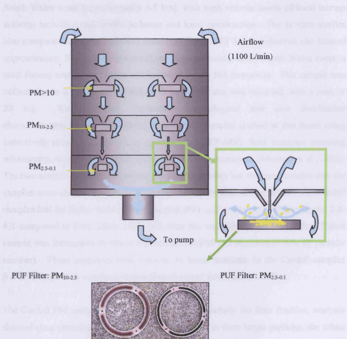
Figure 1.4: A diagram illustrating the mechanisms of the Harvard high volume cascade elutriator PM collector used for the larger scale collection of PM_{10-0.1} for all PM samples described in this thesis. (Moreno et al., 2003)
