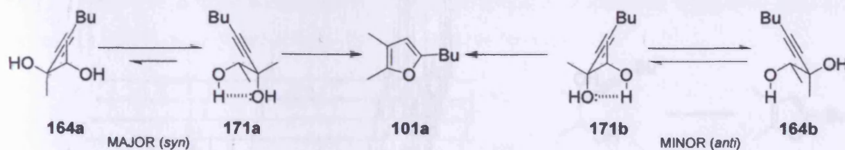
Scheme 43: Cyclisation of syn - 164a and anti - 164b diastereomers.
