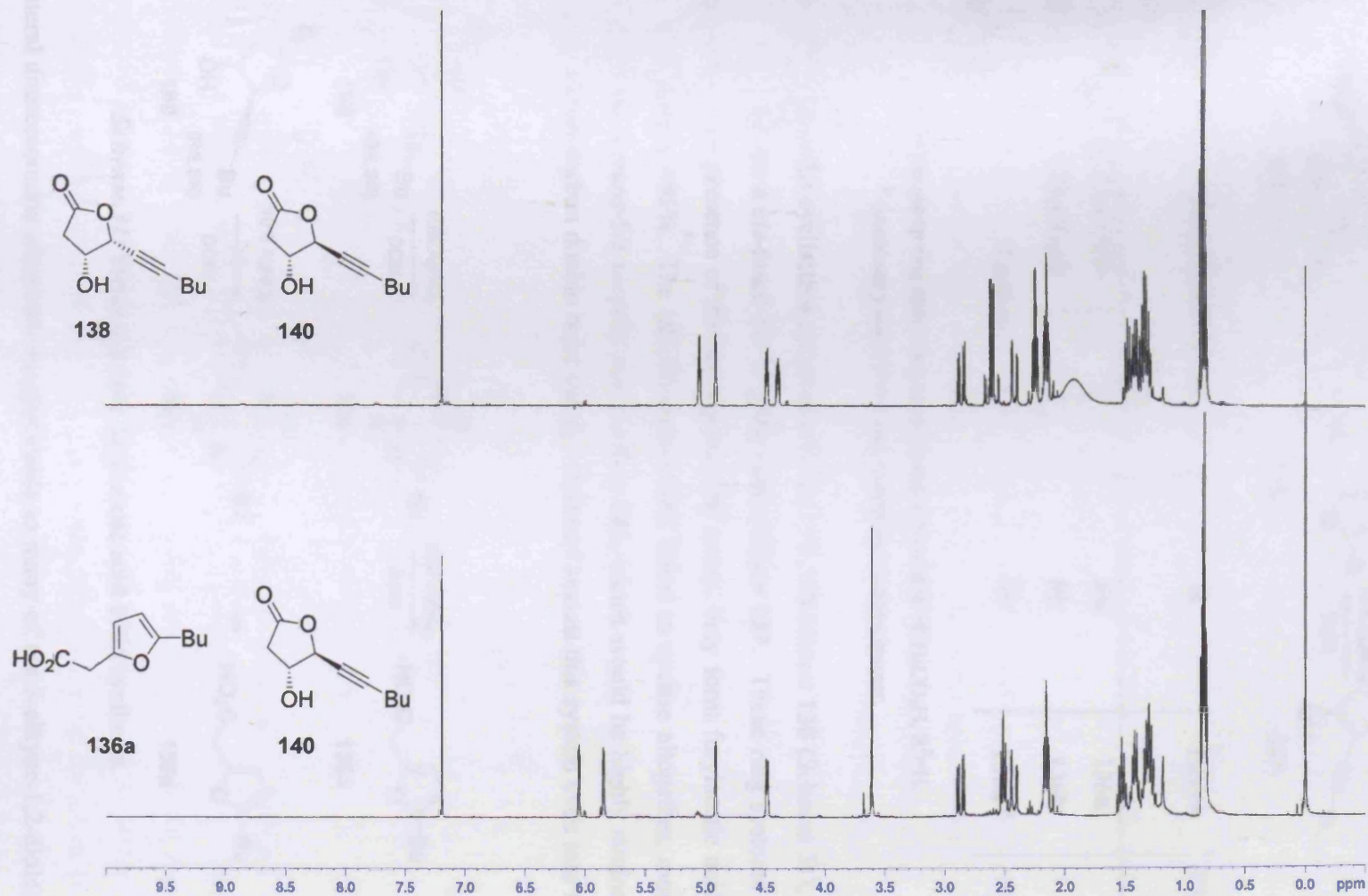
Spectrum 6: 1 H NMR spectrum of lactone 138 and 140 (CDCl 3 ) cyclising to furan 136a (CDCl 3 ).
