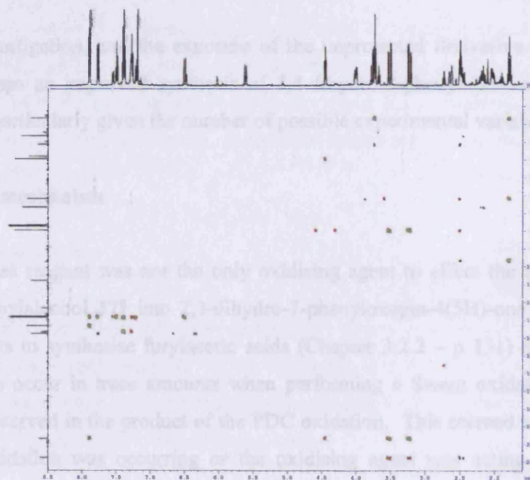
Figure 36: HMBC analysis of 3,4-dihydro-8-phenyloxocin-5-one 397 .
