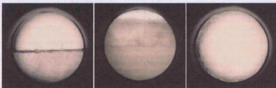
Figure 25: Phase photographs of \text{CO}_2 transforming into \text{scCO}_2 .
