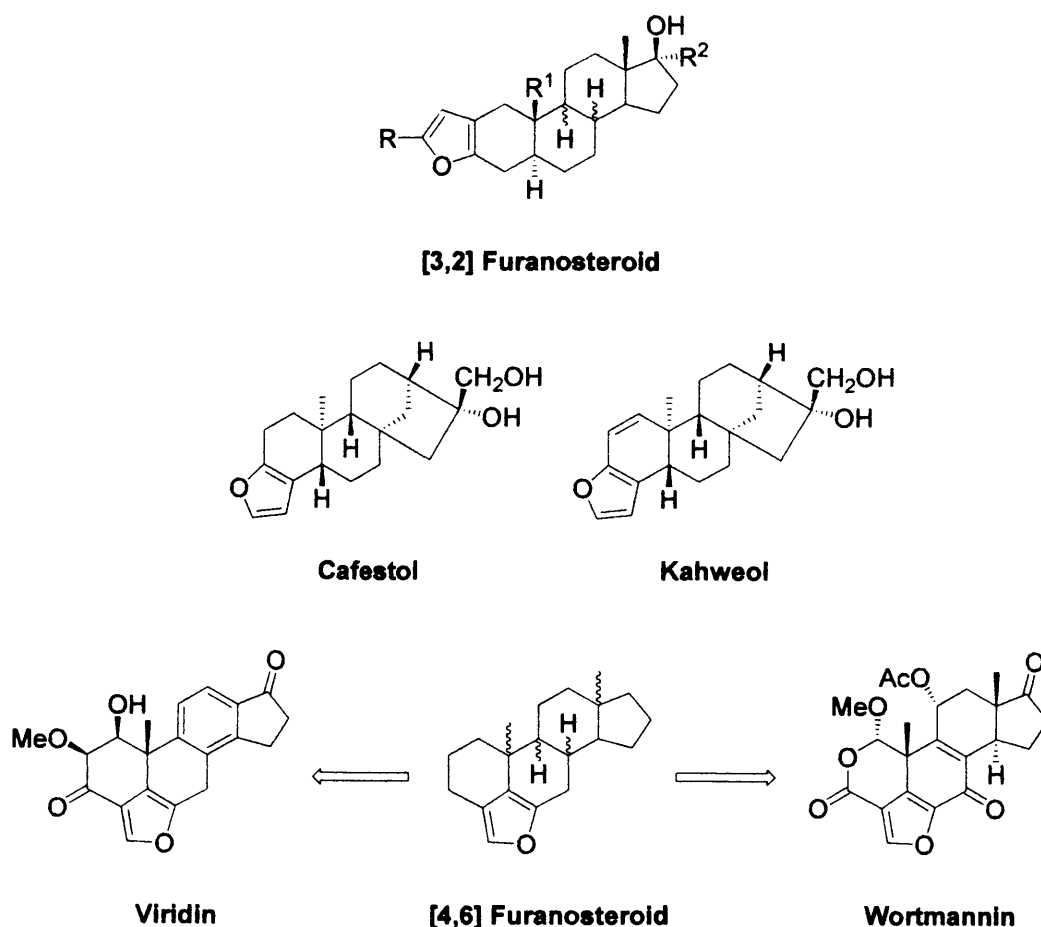
Figure 5: Furanosteroids.
