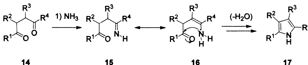
Scheme 5: Paal-Knorr synthesis 5,6 of pyrroles 17 .
