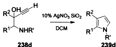
Scheme 66: Synthesis of 2,3-substituted pyrrole 239d .
