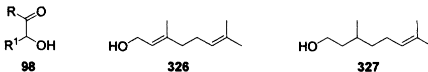
Scheme 103: Core building blocks for synthesis of iso -sesquirosefuran analogues.
