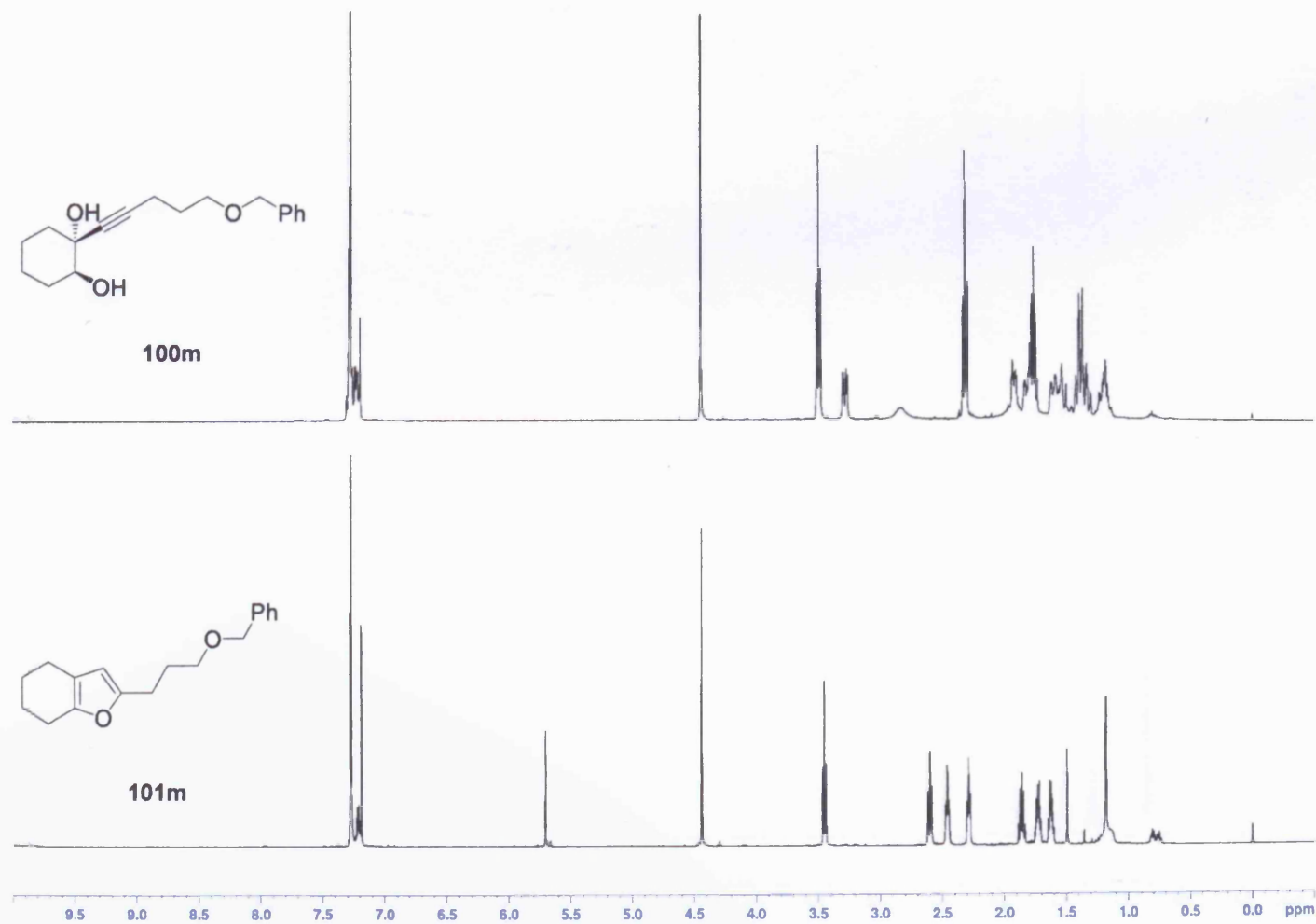
Spectrum 2: 1 H NMR spectrum of diol 100m (CDCl 3 ) and furan 101m (CDCl 3 ).
