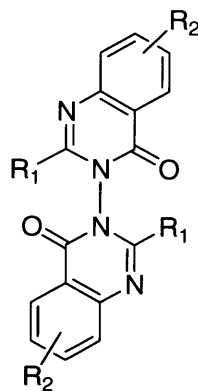
Figure 6.2. Bis(tetrahydroquinazolinones)
