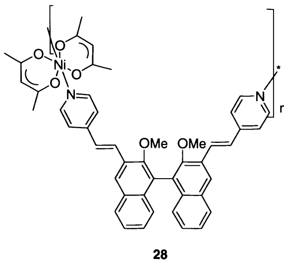
Figure 1.28 Nickel helicate 28
