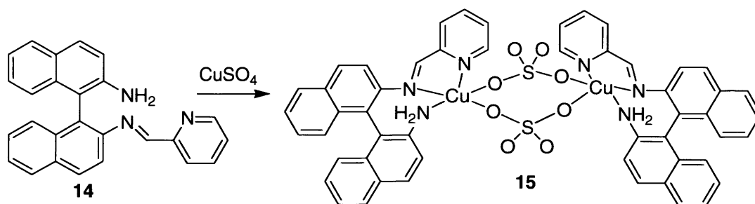
Figure 5.12 [Cu((R)-10)(μ-SO 4 ) 2 ]
