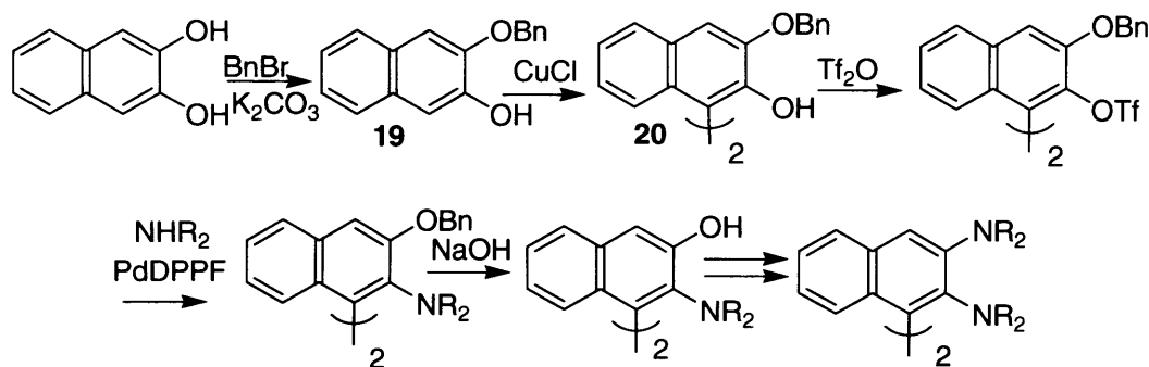
Figure 3.22 Reaction scheme for tetraamine synthesis.
