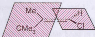
Figure 1.1 An allene with a chiral axis.
