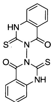
Figure 6.6- Disulphone dione
