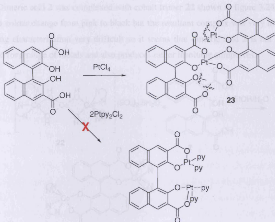
Figure 3.24 Platinum complexes of dimeric acid 2
