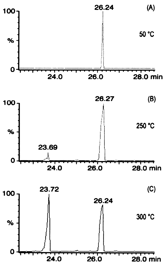
Figure 3.5: GC analysis of the temperature induced reaction products of the pentane extractable products of 2-fluoroFPP (155) from the cyclization by AS. (A) GC analysis of the compound produced by AS from 155 at an injection port temperature of 50 °C. (B) GC analysis of the same compound at an injection port temperature of 250 °C; (C) GC analysis of the same compound at an injector port temperature of 300 °C.
