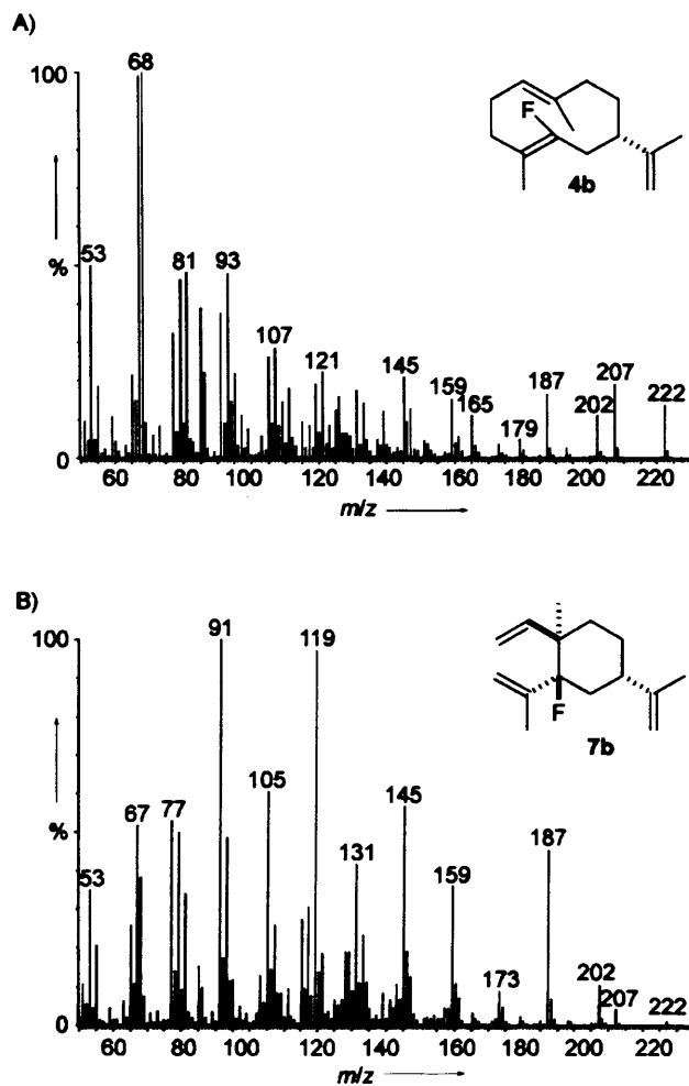
Figure 2. Mass spectral analysis of the two isomers produced by thermal rearrangement in the GC injector. A) EI + Mass spectrum of the material eluted at 26.24 min, which is the presumed 2-fluoro-germacrene A derivative 4b ; B) EI + mass spectrum of the material eluted at 23.72 min, which is the presumed \beta -elemene analogue 7b .
