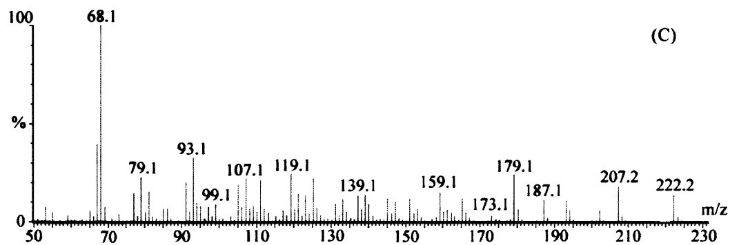
Figure 3.7: GC-MS analysis of the pentane extractable products of 6-fluoroFPP ( 156 ) utilisation by AS, (A) GC analysis of the compounds produced by AS from 156 at an injection port temperature of 50 °C; (B) EI^+ mass spectrum of the material eluting at 26.81 min; (C) EI^+ mass spectrum of the material eluting at 27.48 min.
