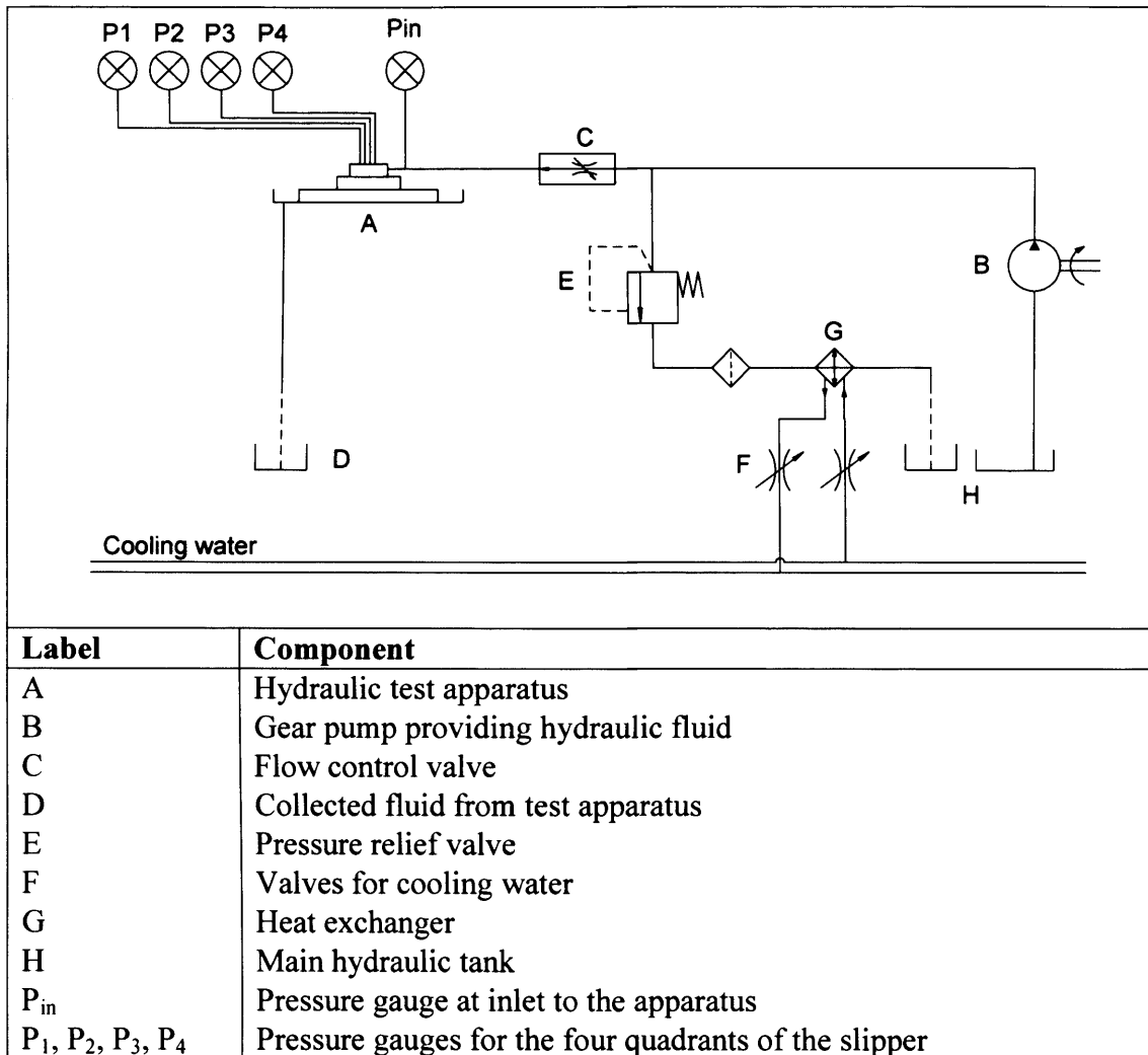
Figure 4.13 Hydraulic circuit
