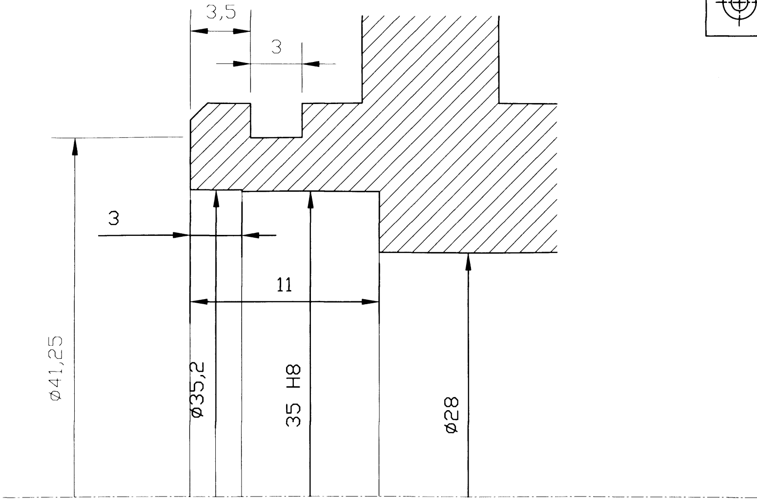
Detail of seal seat, drawing JMH009A
