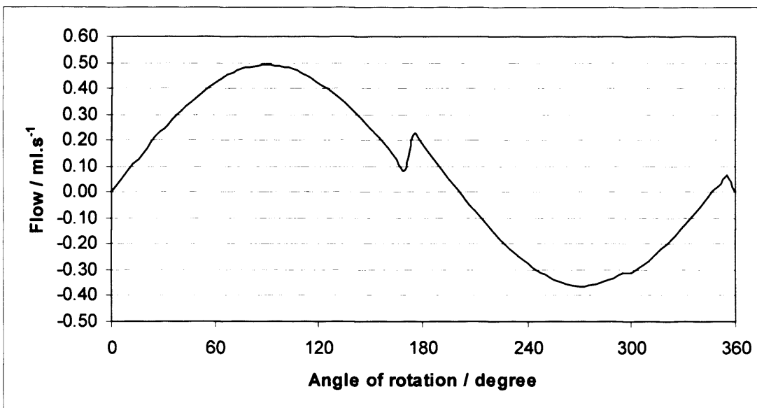
Figure 3.24 CFD derived flow through the gap between a piston and its bore, radial clearance of 10 \mu m
