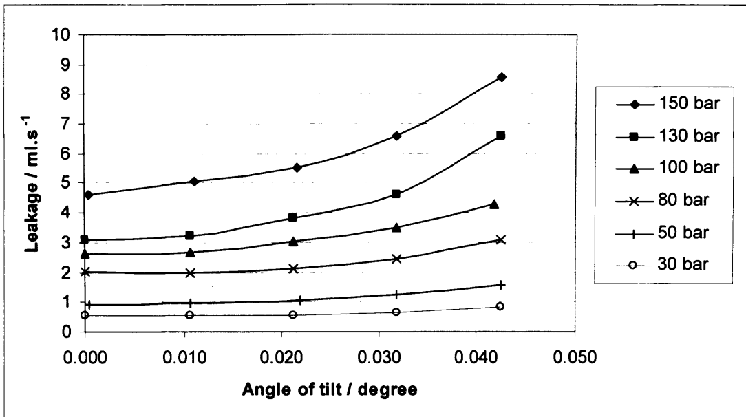
Figure 4.24 Leakage characteristics at a central clearance of 20µm
