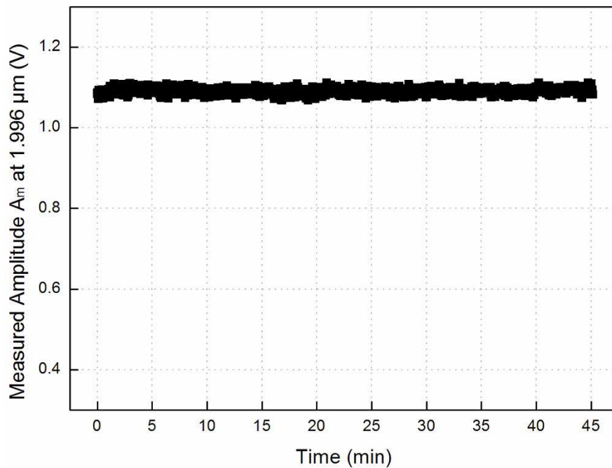
Fig. 7.8 Stability of the \text{Tm} -doped fibre laser based gas sensor system over time
