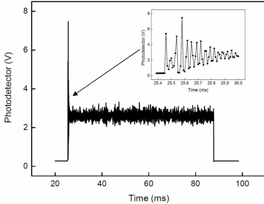
Fig. 7.5 Transient behaviour of Tm-doped fibre laser
