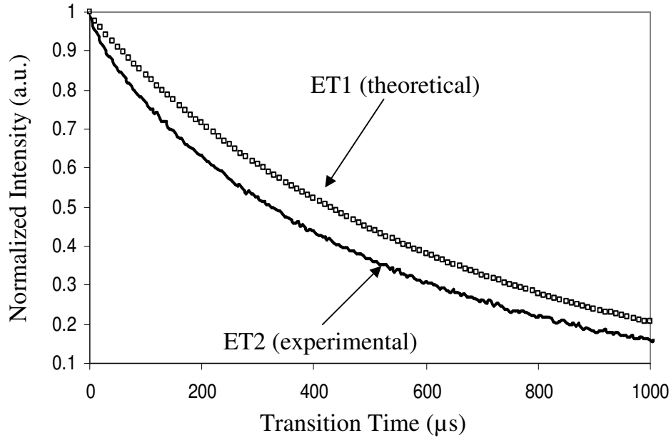
Fig. 4.10 Normalized decay curves for {}^2F_{5/2} level in TYDF-A-4 considering first step energy-transfer (theoretical) and second step energy-transfer (experimental)
