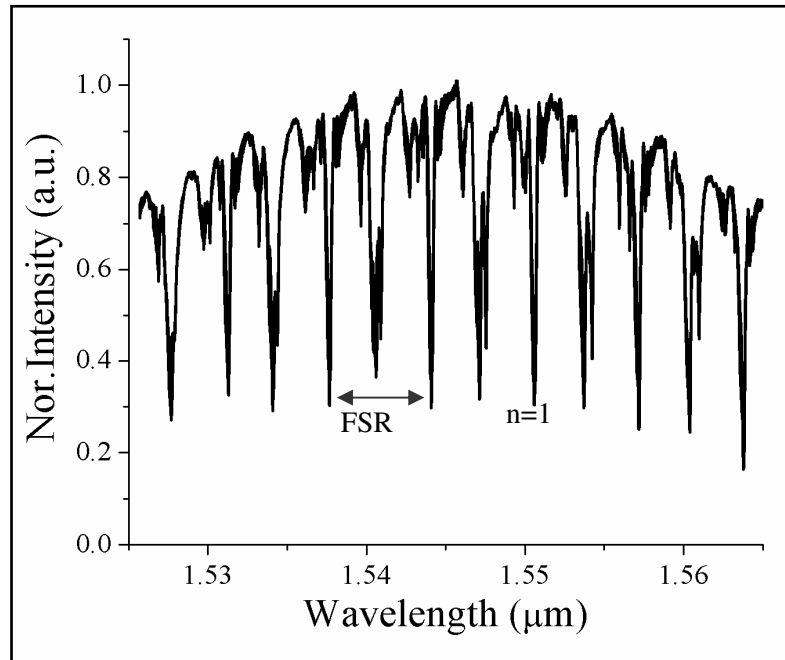
Fig. 6.11 Resonances in the microsphere coupled with a tapered fibre
