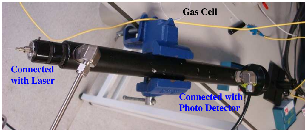
Fig.7.3 Images of Tm-doped tuneable fibre laser and gas cell used in sensor system
