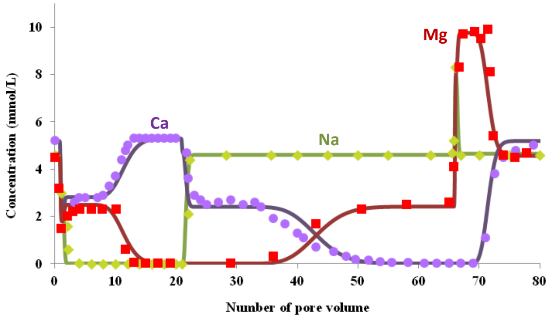
Figure 5: Comparison of the experimental BTCs reported by Voegelin et al. (2000) and obtained with a B soil horizon with those predicted using our model based on the sorption properties of Wyoming montmorillonite. The data correspond to experiment 1 in the study by Voegelin et al. The details of the prediction are provided in the text.
