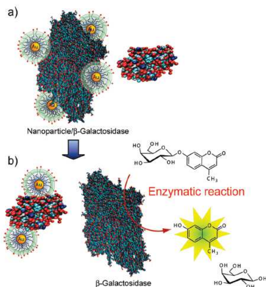
Figure 1.38. Enzyme-amplified sensing array. a) Functionalized cationic AuNPs electrostatically bind to the anionic \beta -Galactosidase ( \beta -Gal), reversibly inhibiting the enzyme. b) Displacement of the particles by the analyte restores \beta -Gal activity toward a fluorogenic substrate, generating a readout signal that is amplified through enzymatic catalysis. [95]
