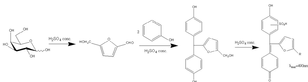
Figure 5.20. Reaction mechanism: in concentrated acid media, galactose is dehydrated and produces 5-hydroxymethylfurfural, which, in the presence of phenol, gives a colored substance showing a maximum of absorbance at \lambda = 490 nm.
