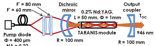
Fig. 3 Experimental setup
