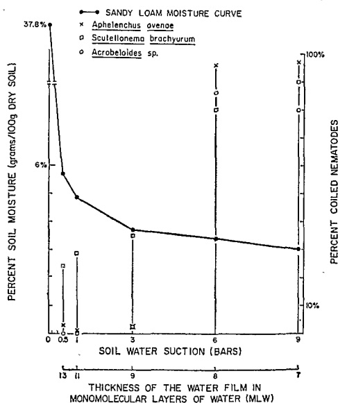
FIG. 3. Soil moisture characteristic of a sandy loam (72.8% sand, 21.2% silt, and 6% clay) and percentage of coiling of A. avenae (x), S. brachyurum (□) and Acrobeloides sp. (o).
