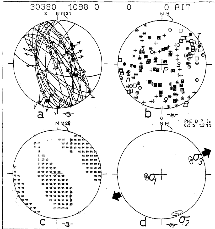
Fig. 7. Example of a detailed analysis of a population of faults, Gloria and Inferno Formations, Arroyo Soledad, Santa Rosalia Basin. Schmidt's projection, lower hemisphere. (a) Fault planes and slickenside lineations and poles to stratification. (b) Axes related to individual fault mechanisms (n, poles to fault planes, s, slickenside lineations, B, P, and T, axes of earthquake focal mechanisms solutions). (c) Diagram of the method of right dihedral angles which define mechanical compatibilities between all faults (Angelier & Mechler 1977). Small numbers are frequencies (percentages) for maximum compressive stress ( \sigma_1 ), large numbers are frequencies for minimum stress ( \sigma_3 ), (d) result of the inversion of data. The axes of the computed stress tensor are plotted ( \sigma_1, \sigma_2, \sigma_3 ). Large arrows show the direction of extension. Methods are described in detail in Angelier (1979). The mathematical inversion of data was also done using a new method (Tarantola et al. in preparation).
