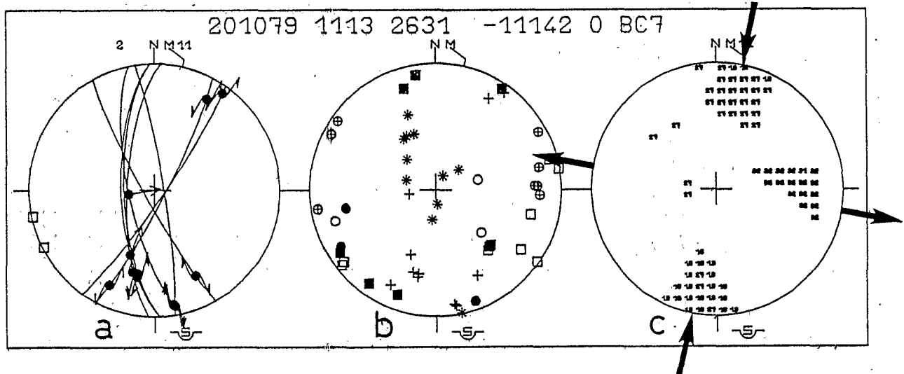
Fig. 12. Conjugate strike-slip faults in the Comodu Formation (Bahia Concepcion). For legend see Fig. 7.
