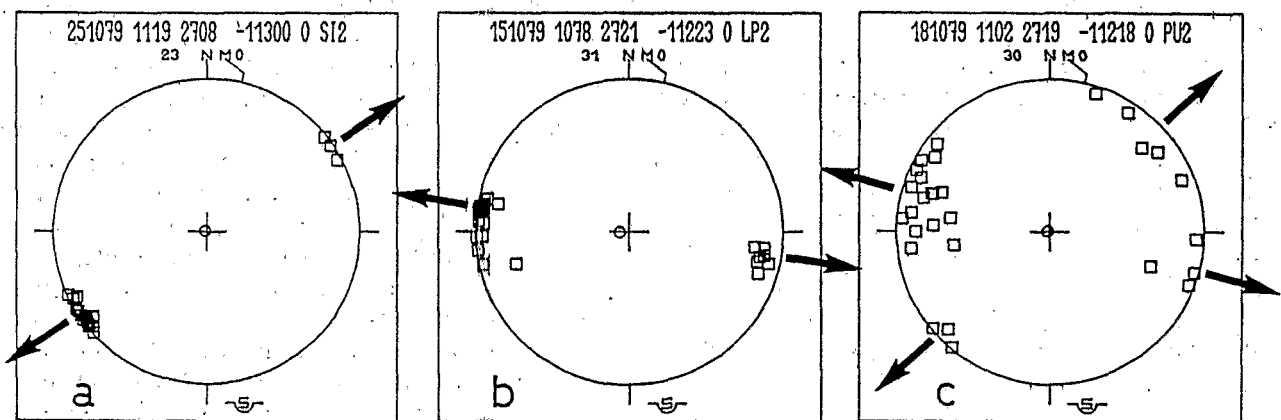
Fig. 11. Examples of populations of tension gashes. (a) San Ignacio. (b) Las Palmas, Santa Rosalia Basin. (c) Arroyo Purgatorio, Santa Rosalia Basin. Squares are poles to tension gashes, open circles are poles to bedding.
