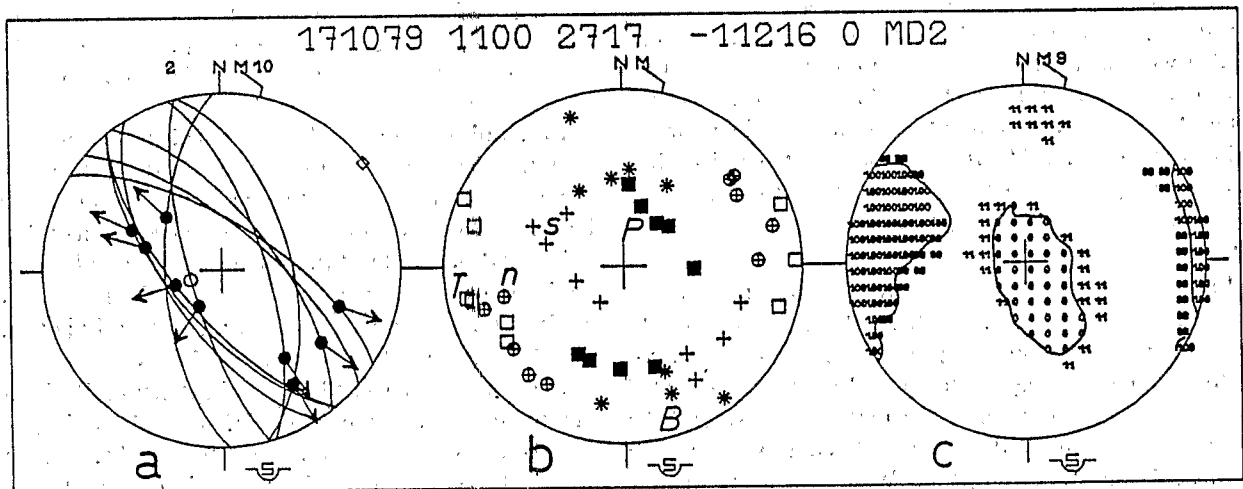
Fig. 9. Normal dextral oblique-slip faults (Ojoria Formation, Arroyo Montado, Santa Rosalia Basin). For legend see Fig. 7.
