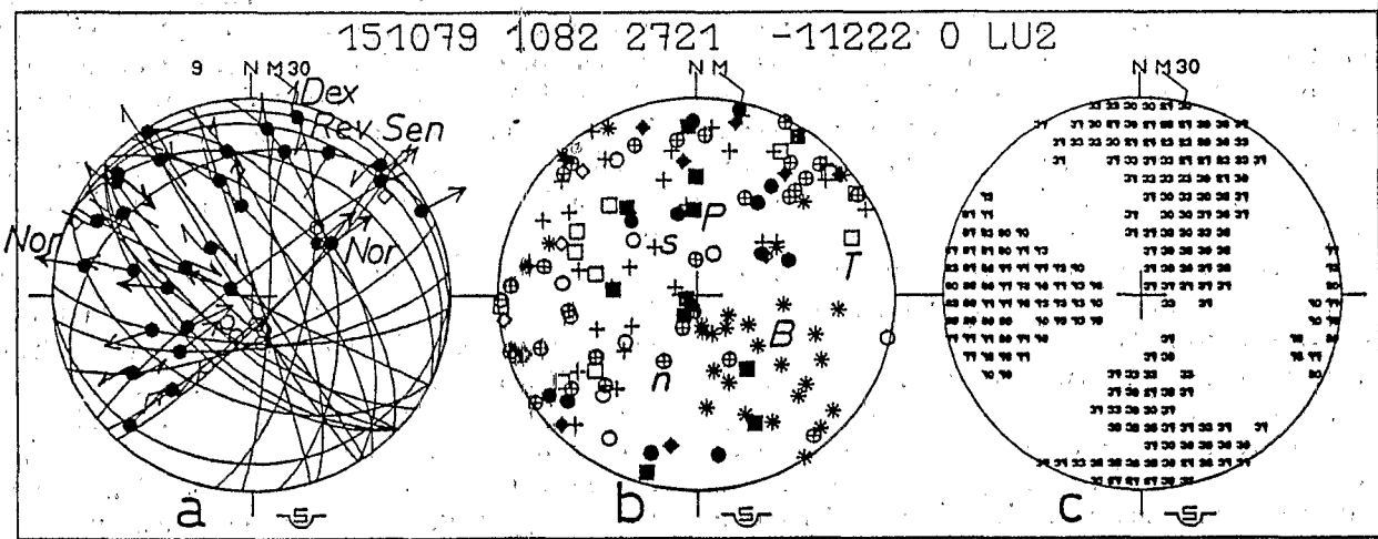
Fig. 13. Complex fault pattern in the Boleo Formation near Mina Lucifer (Arroyo Infierno, Santa Rosalia Basin). For legend see Fig. 7. Dex- and Sen-dextral and sinistral strike-slip faults respectively, Rev, reverse faults; Nor, normal faults.
