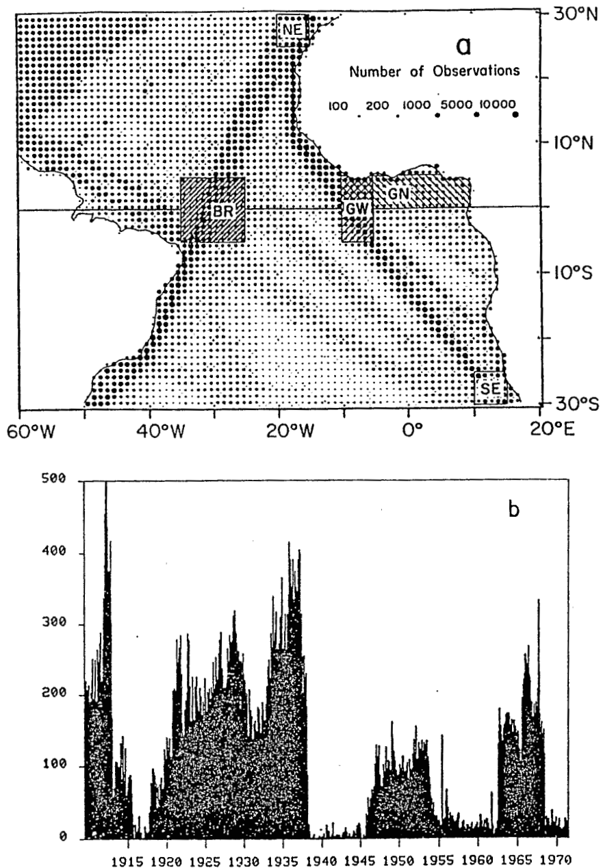
FIG. 1. (a) Position of the studied areas (composite picture from Hastenrath and Lamb, 1977). (b) Number of observations by month in a part of the BR area ( 0-5^{\circ}\text{S} , 30-35^{\circ}\text{W} ).
