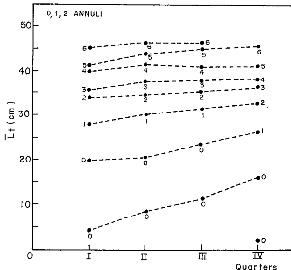
FIG. 3. — Average length of females with the same number of annuli on the scales in function of trimester
