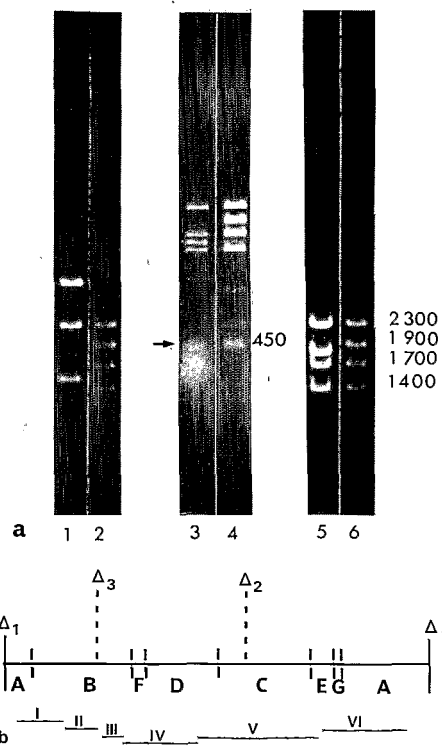
Fig. 3. Genomes of the different strains used. Viral strains S and CM4.184 correspond to the hybrid DNA molecules pCaBT37 and pCaDavis20 as described in Materials and methods. \Delta 1 , \Delta 2 , \Delta 3 represent the three gaps in strain S DNA (Volovitch et al. , 1978). Unshaded and black segments represent the double-stranded DNA from the S (8024 bp) and CM4.184 (7610 bp) strains, respectively. Numbers indicate the eight ORFs (Hohn et al. , 1982). Construction of the S.ΔII mutant. Nucleotides 1534–1642 were deleted (see Materials and methods), and a 16 bp long insert was introduced in the XhoI (◆) site. Note that the original reading frame is maintained. The potential translation product would have a mol. wt. of 15 kd (potential protein pP15). The partial nucleotide sequence of the insertion fragment is indicated in the blown-up form. Nucleotides 1534–1537 are common in the S.ΔII and strain S. Construction of the S.CM4 recombinant strain: a large BstEII (■, position 126)- BamHI (▼, position 1926) restriction fragment of S and the small one of CM4.184, BstEII (■, position 126)- BamHI (▼, position 1505) were joined by ligation.
