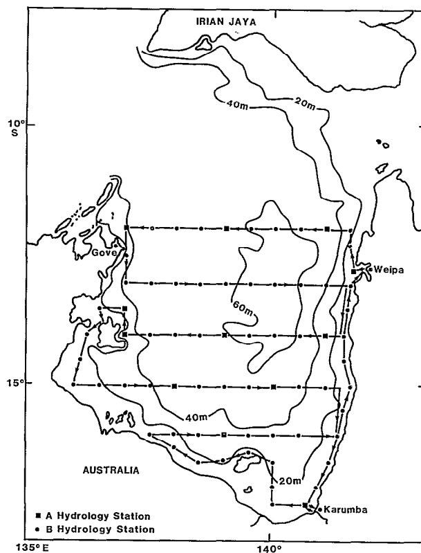
FIG. 1. — Location and bathymetry (depth in metres) of the Gulf of Carpentaria. A sample cruise track shows hydrology sampling stations
