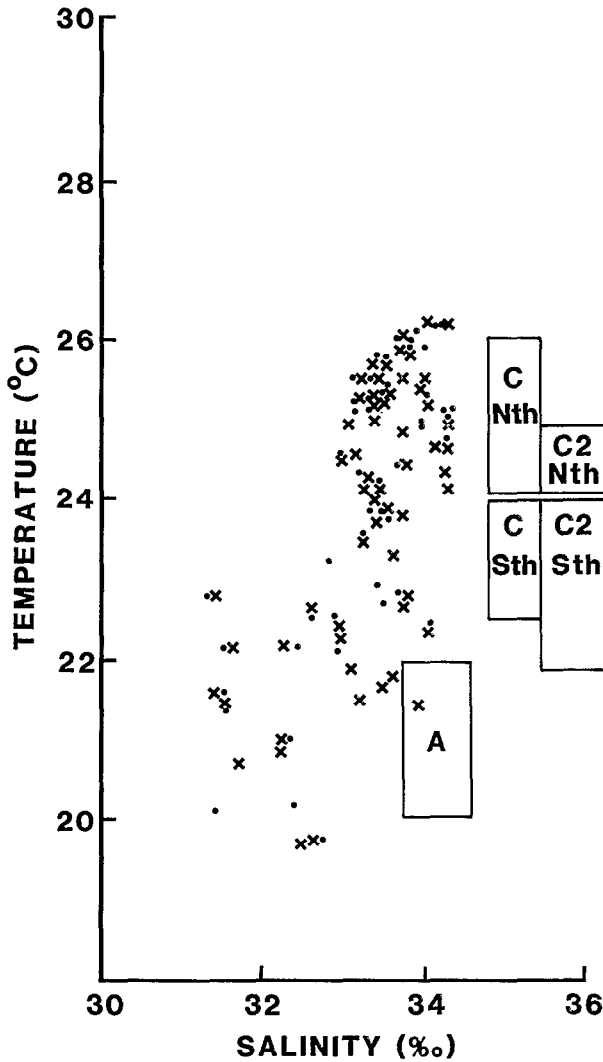
FIG. 2. — T.S. (Temperature vs. Salinity) diagram for winter. In Figures 2, 3, 4 and 5 (●) are surface values and (X) deep values for the whole of the Gulf; previously identified water masses are enclosed by boxes; "Sur" and "Bot" indicate different characteristics in surface and bottom water and "Sth" and "Nth" indicate southern and northern regional differences
