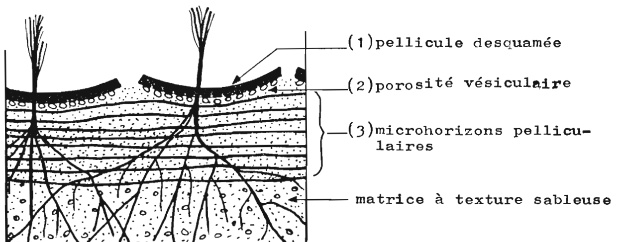
Type 46 SURFACE A PELLICULE REBROUSSEE
