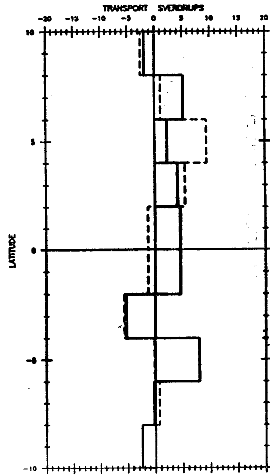
US/PRC CRUISE 3 OCTOBER 1987
