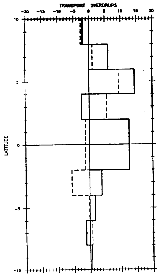
US/PRC CRUISE 2 DECEMBER 1986
