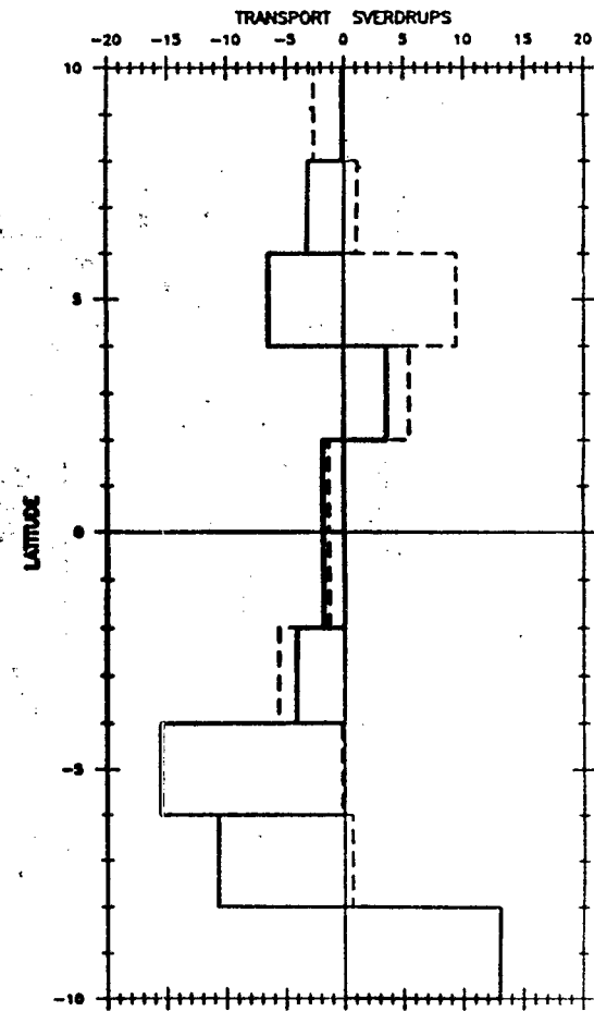
US/PRC CRUISE 4 MAY 1988
