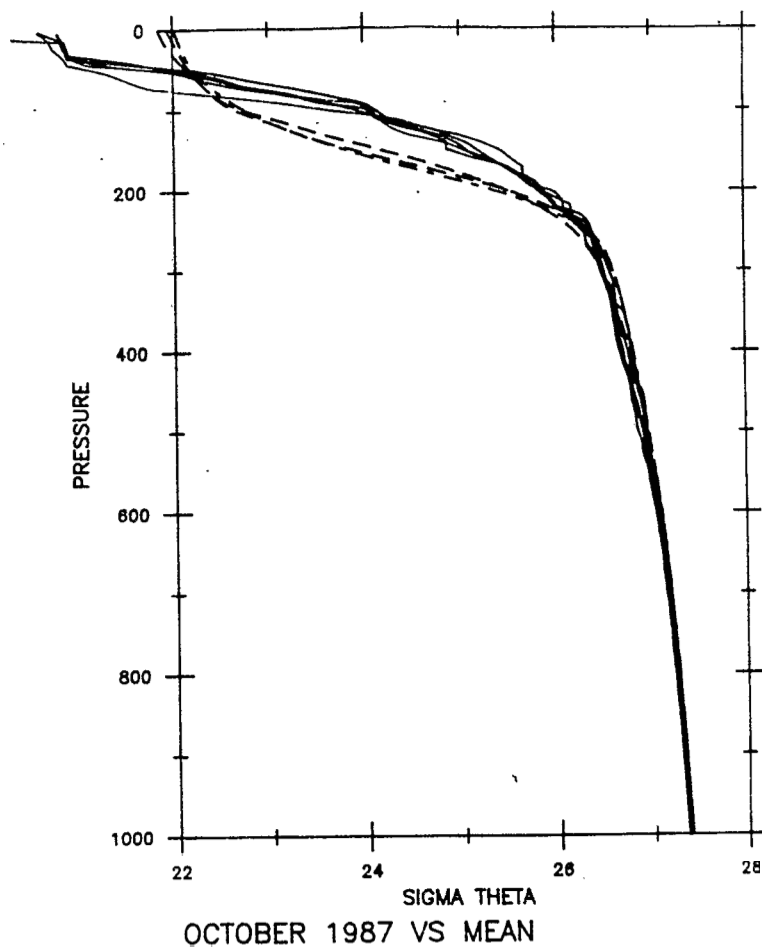
Fig.5. Profiles of potential density between 2° N and 2° S observed in October 1987 (solid lines) and the annual mean profiles (dashed lines)
