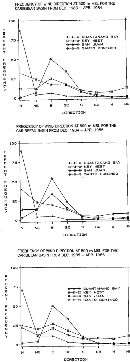
Fig. 4. Wind direction frequency (%) for the southeastern U.S. and the Caribbean Basin (Top) Dec. 1983 - Apr. 1984, (Middle) Dec. 1984 - Apr. 1985, and (bottom) Dec. 1985 - Apr. 1986.
