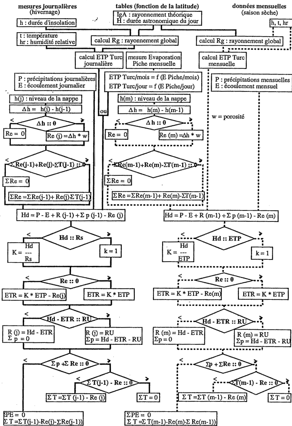
Fig. 5. - Organigramme du bilan hydrique (Organigram of the moisture balance)
