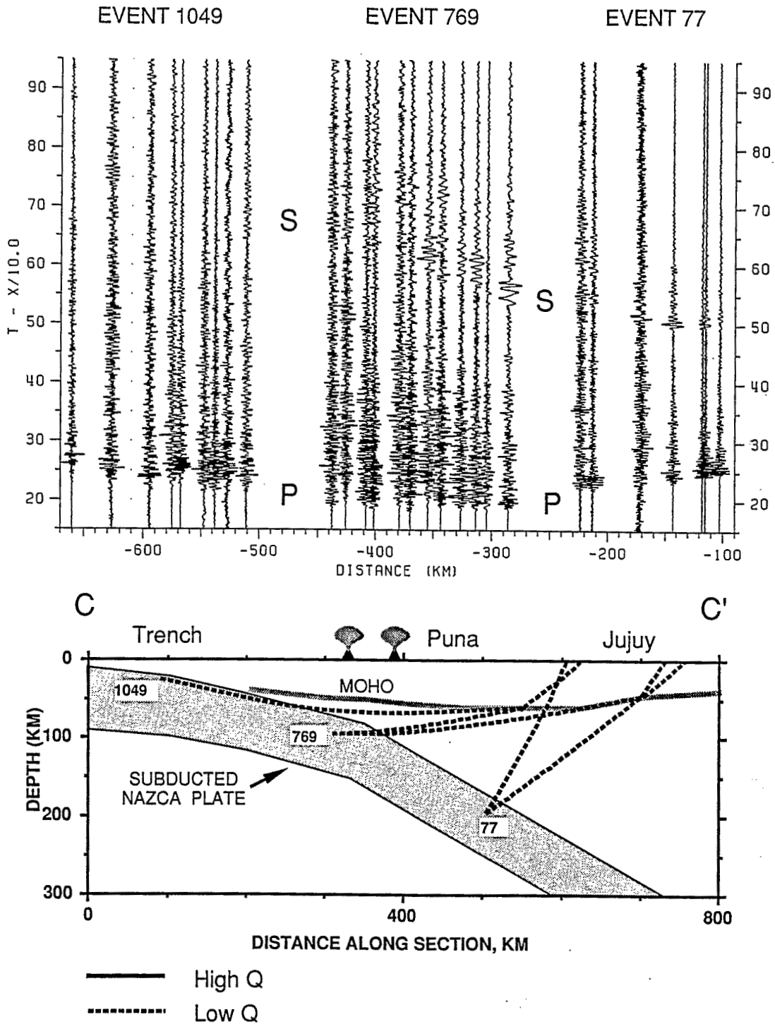
Fig. 8. Interpretive cross section and composite radial component record section constructed along line C-C' in Figure 2. Event numbers correspond to labeled earthquakes in Figure 2. Section is roughly perpendicular to the strike of the Plateau. Events 77 and 769 both contain only low-frequency S waves. S waves for event 1049 are of an indeterminate nature, indicating high scattering and attenuation for the path beneath the whole width of the Andes.
