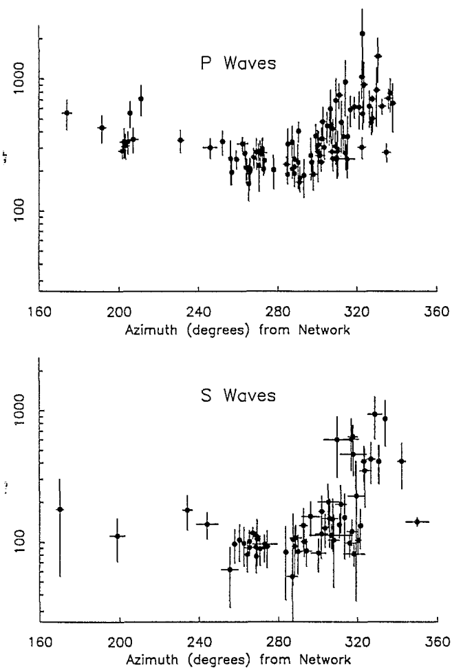
Fig. 5. Plot of the average apparent Q for each WBZ earthquake observed at the Jujuy network versus observed azimuth estimated from travel time slowness measured across the network. Vertical and horizontal error bars denote \pm 1 standard deviation for each Q average and the estimated standard error of each slowness measurement, respectively.
