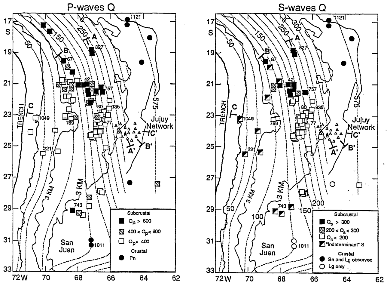
Fig. 2. Estimated apparent Q for P (left) and S (right) wave ray paths to the Jujuy network. Map shows shape of the subducted Nazca plate (labeled contours) [after Cahill, 1990, Cahill and Isacks, 1992], 3-km average elevation contour, and locations of earthquakes used in the attenuation study. Earthquake locations are from the PDE and ISC. Numbered earthquakes are events referred to in the subsequent figures. Note that events producing high- Q ray paths (dark shaded circles and squares) are all located to the north and northwest of the Jujuy network (small triangles).
