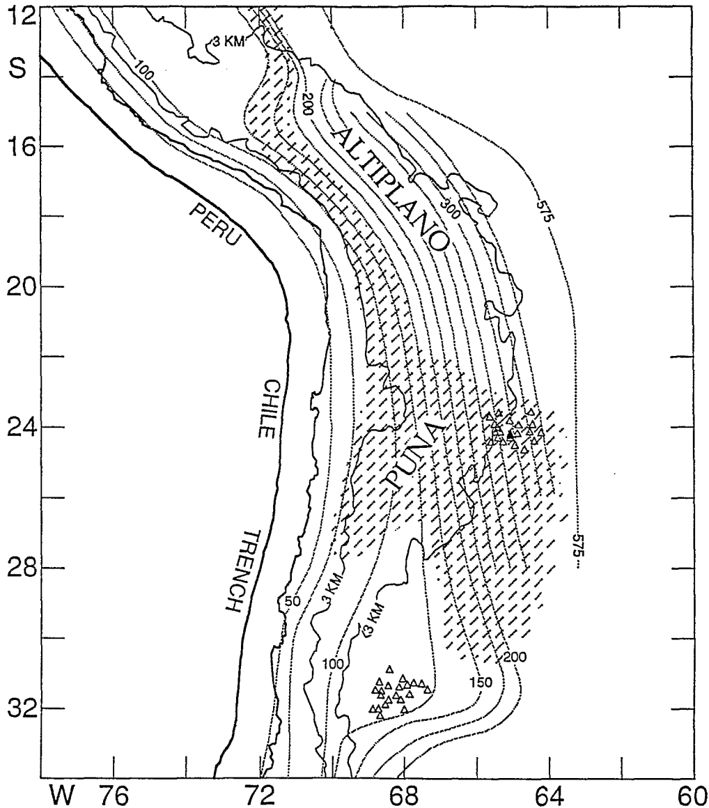
Fig. 12. Map showing regions of high seismic wave attenuation (shaded region) inferred to lie between the subducting Nazca plate and the overriding South American plate. Also shown is depth to the Wadati-Benioff zone [Cahill and Isacks, 1992] and the average 3-km topographic elevation contour.
