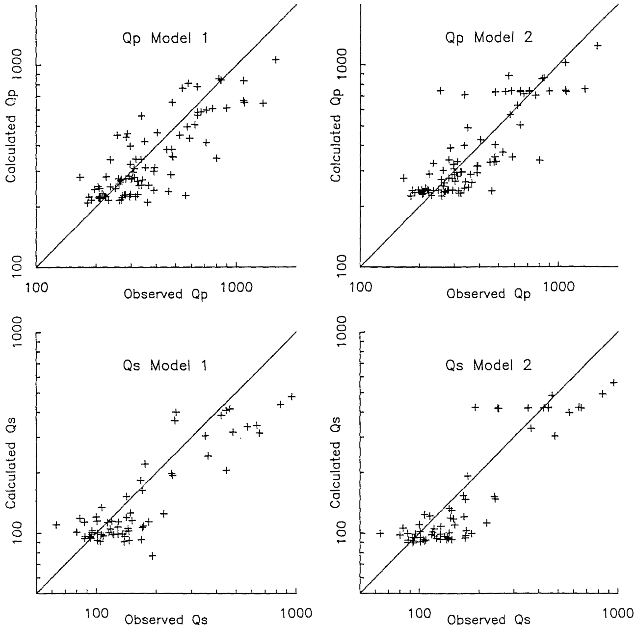
Fig. 16 . Scatter plot comparing average observed Q for each event and the calculated average event Q for models 1 and 2. The calculated values generally fall within 30% of the observations.
