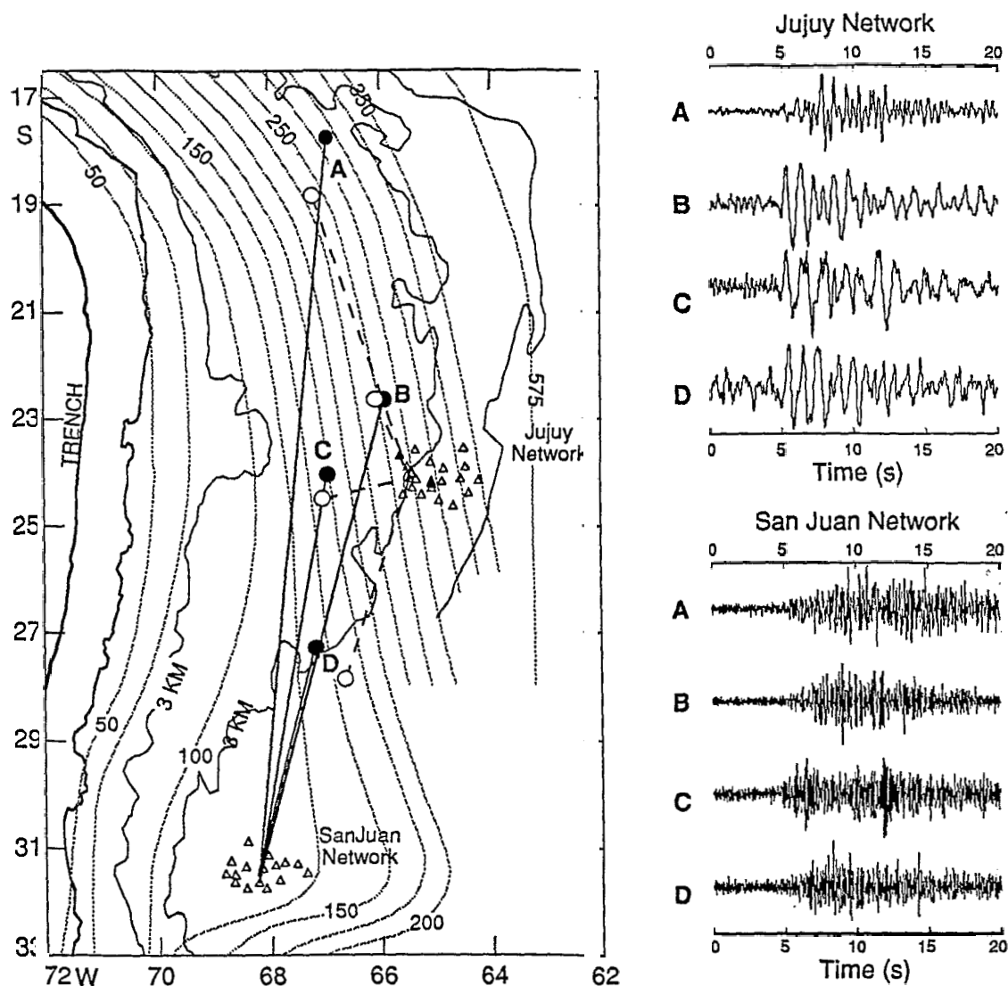
Fig. 10. Comparison of radial component shear waves from intermediate-depth earthquakes recorded at the PANDA San Juan and Jujuy networks (triangles). Events recorded at the San Juan array (solid circles) produce high-frequency shear waves which are guided along a continuous high- Q subducted lithosphere, while lower frequency shear waves are recorded at the Jujuy network.
