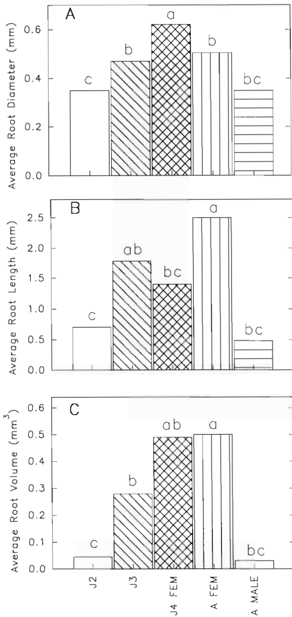
Fig. 2. A : Mean root diameters, as measured at the head of the nematode, occupied by the different stages of Heterodera schachtii within sugarbeet roots; J2 = second-stage juvenile; J3 = third-stage juvenile; J4 FEM = fourth-stage female; A FEM = adult female; and A MALE = fourth-stage male. Means represented by columns with different letters above them are significantly different as judged by pairwise t -test comparisons ( p = 0.05 ). – B : Mean root lengths occupied by the different stages of Heterodera schachtii within sugarbeet roots. J2 = second-stage juvenile; J3 = third-stage juvenile; J4 FEM = fourth-stage female; A FEM = adult female; and
