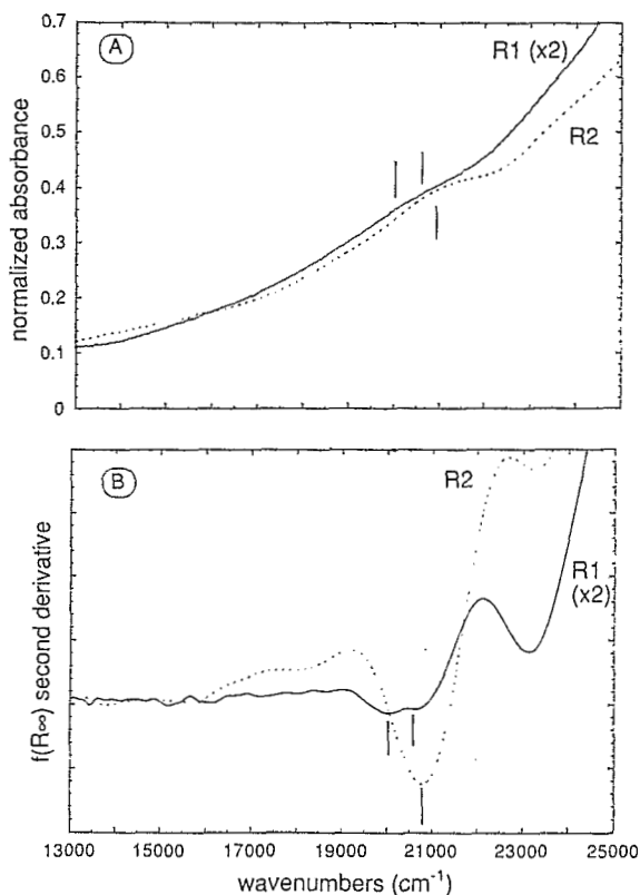
Figure 6. Raw spectra (A) and second derivative curves (B) of bleached soil samples (R1, R2) in the visible range. Remission function values for R1 have been multiplied by two for a better comparison of features with R2 sample. The band near 23,400 \text{cm}^{-1} is characteristic of goethite. The vertical bars on (A) indicate the positions of diagnostic bands determined from second derivative curves.
