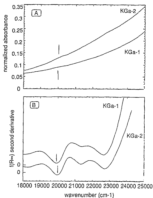
Figure 7. Raw spectra (A) and second derivative curves (B) in the absorption region ( 18,000\text{--}25,000\text{ cm}^{-1} ) of bleached sedimentary kaolins (KGa-1, KGa-2) immersed in paraffin oil. The two bands near 21,000\text{ cm}^{-1} and 23,000\text{ cm}^{-1} are likely due to Fe-bearing anatase. The vertical bars on (A) indicate the positions of diagnostic bands determined from second derivative curves.
