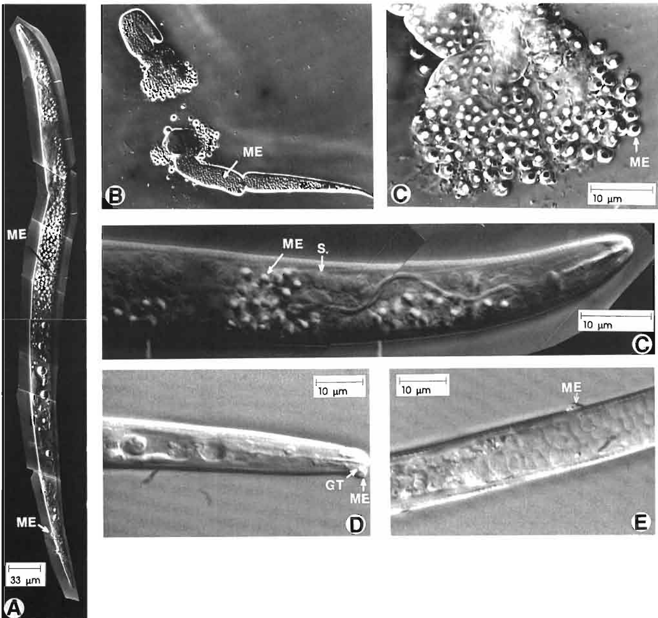
Fig. 1. Second-stage juveniles (J2) and males of Tylenchulus semipenetrans parasitized by Pasteuria sp. A : J2 with mature endospore (ME) attached to tail and containing mature endospores and sporangia; B : Pasteuria sp. -filled J2 broken to release mature endospores (ME); C : Detail of mature endospores released from broken J2; D : Asynchronous development of Pasteuria sp. within the J2 as evidenced by sporangia (S) and mature endospores (ME); E : Mature endospore (ME) attached to head region of male T. semipenetrans with germ tube (GT); F : Mature endospore (ME) attached to male cuticle in vicinity of spermatocytes.
