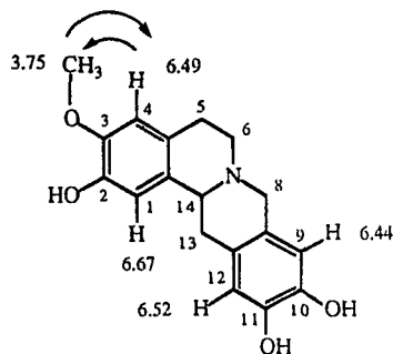
Figure 1. ^1\text{H-NMR} chemical shifts and NOEs of pessoine (1).
