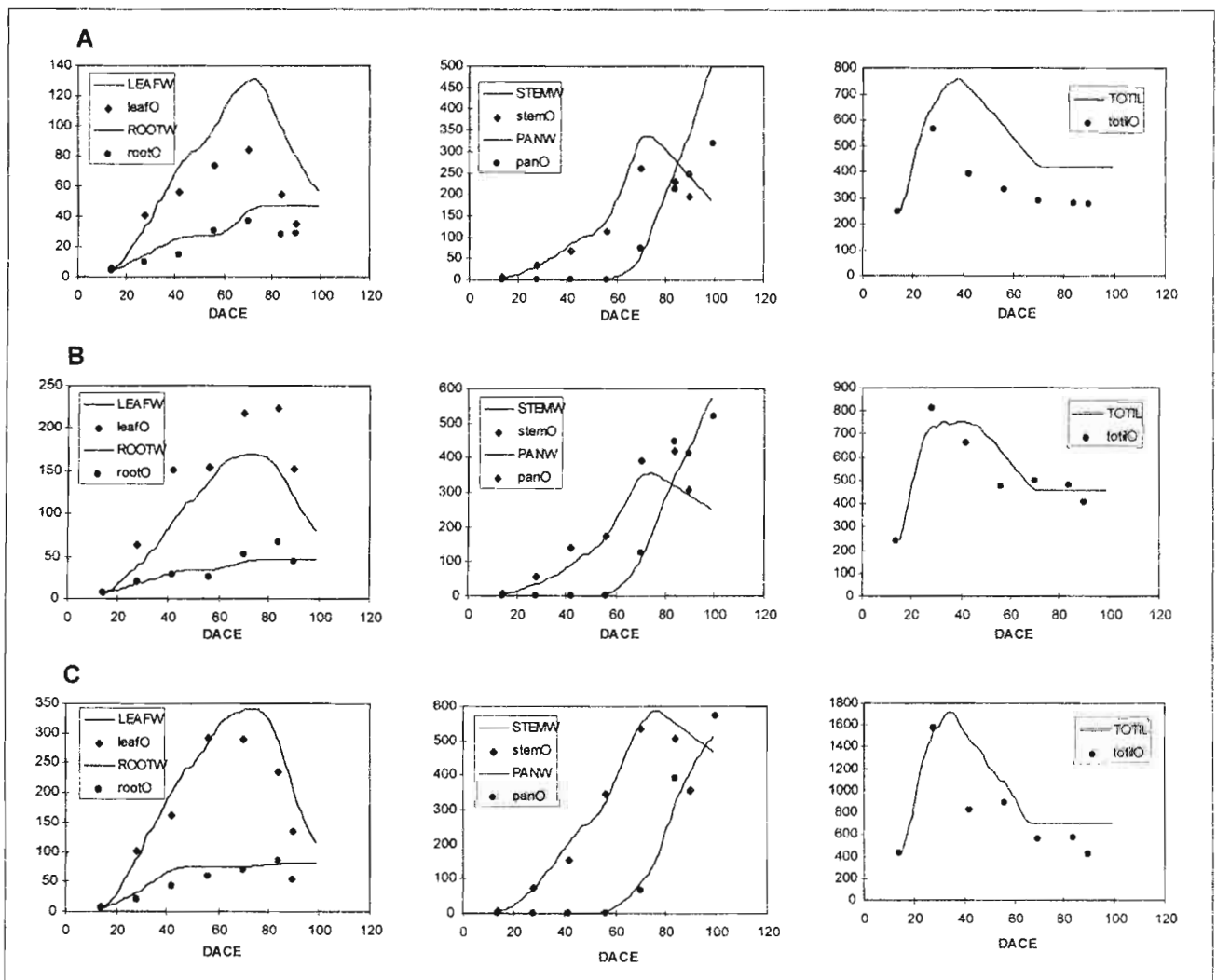
Fig. 22. Rice growth damaged by weeds in three PS: observed (•,*) and simulated (-) dry weight of rice organs, and tiller number. Observed data were collected from the experiment done at IRRI in 1997, WD plots (see text for details). A: PS1; B: PS2; C: PS3.
