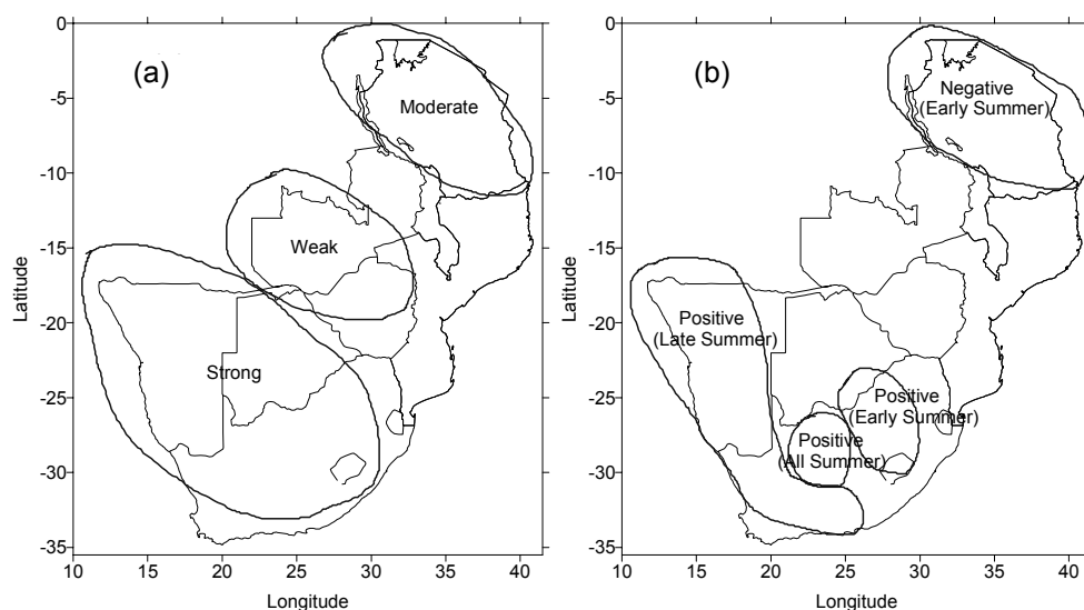
Fig. 3 Generalization of the ENSO-southern African rainfall relationships according to: (a) strength and (b) seasonality and sign of the association with SOI.
