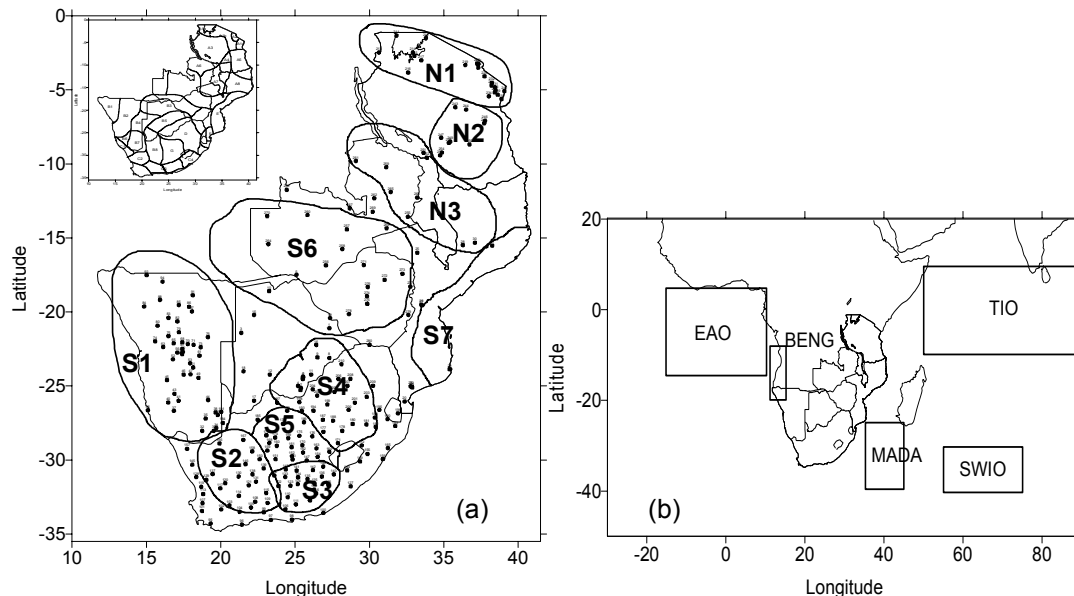
Fig. 2 (a) General coherent clusters from PCA and correlation analysis (Valimba, 2005). (b) Selected oceanic regions in the Atlantic and Indian oceans (Valimba, 2005).
