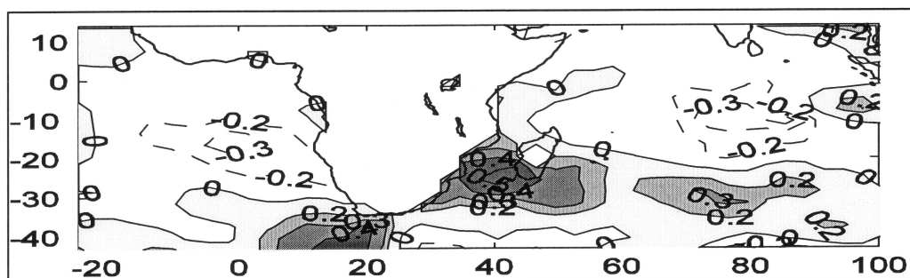
Fig. 5 Correlations between OND SST and S6 (Zambezi) regional ONDJ seasonal amounts. All correlations exceeding 0.39 are significant at 95%.
