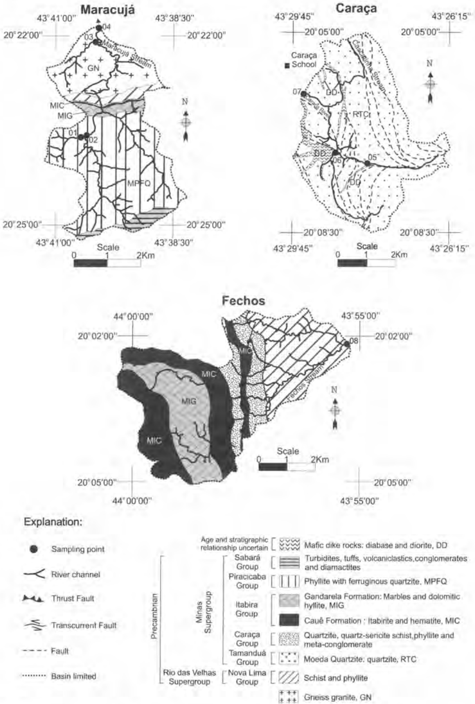
Fig. 2. Geology of studied basins (JOHNSON 1962, POMERENE 1964, MAXWELL 1972).
