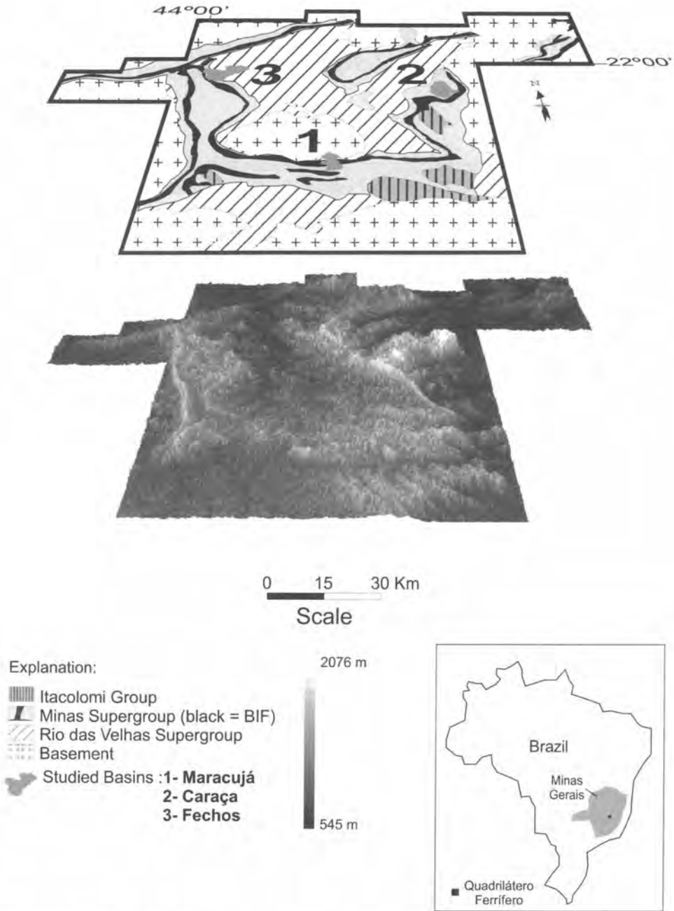
Fig. 1. Quadrilátero Ferrífero geology (ALKMIN & MARSHAK 1998) and relief.
