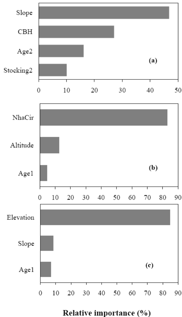
Figure 4.2 Bar charts giving the relative importance of predictor variables determined by BRT approach and used for estimation of C stock in (a) ABG pool, (b) BLG pool and (c) SOC pool.
