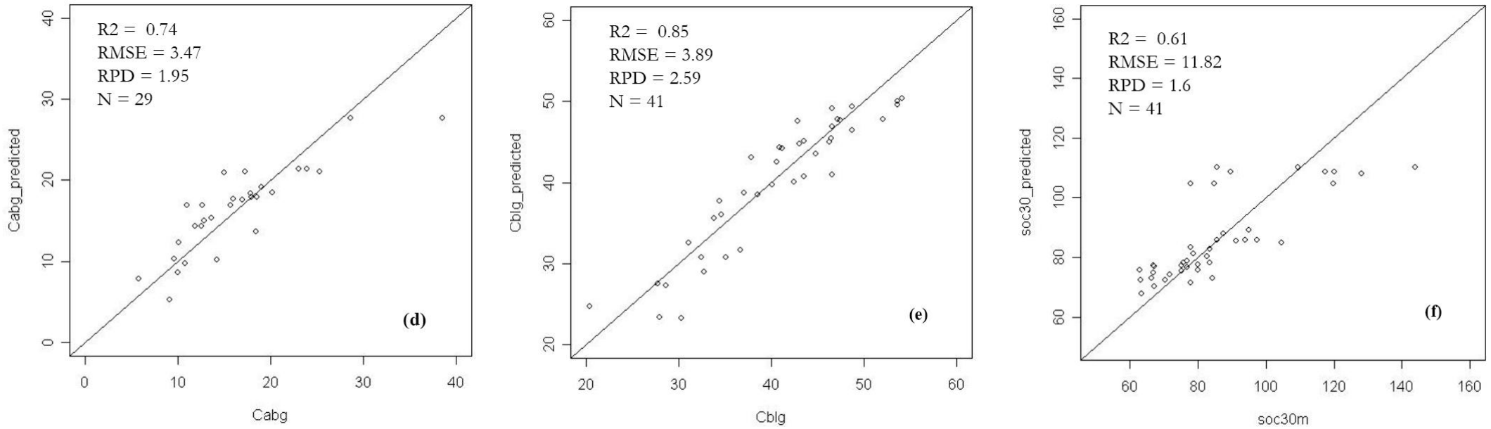
Figure 4.3 Graphs of Predicted vs Measured C stocks for each model retained in (d) ABG pool, (e) BLG pool and (f) SOC pool.
