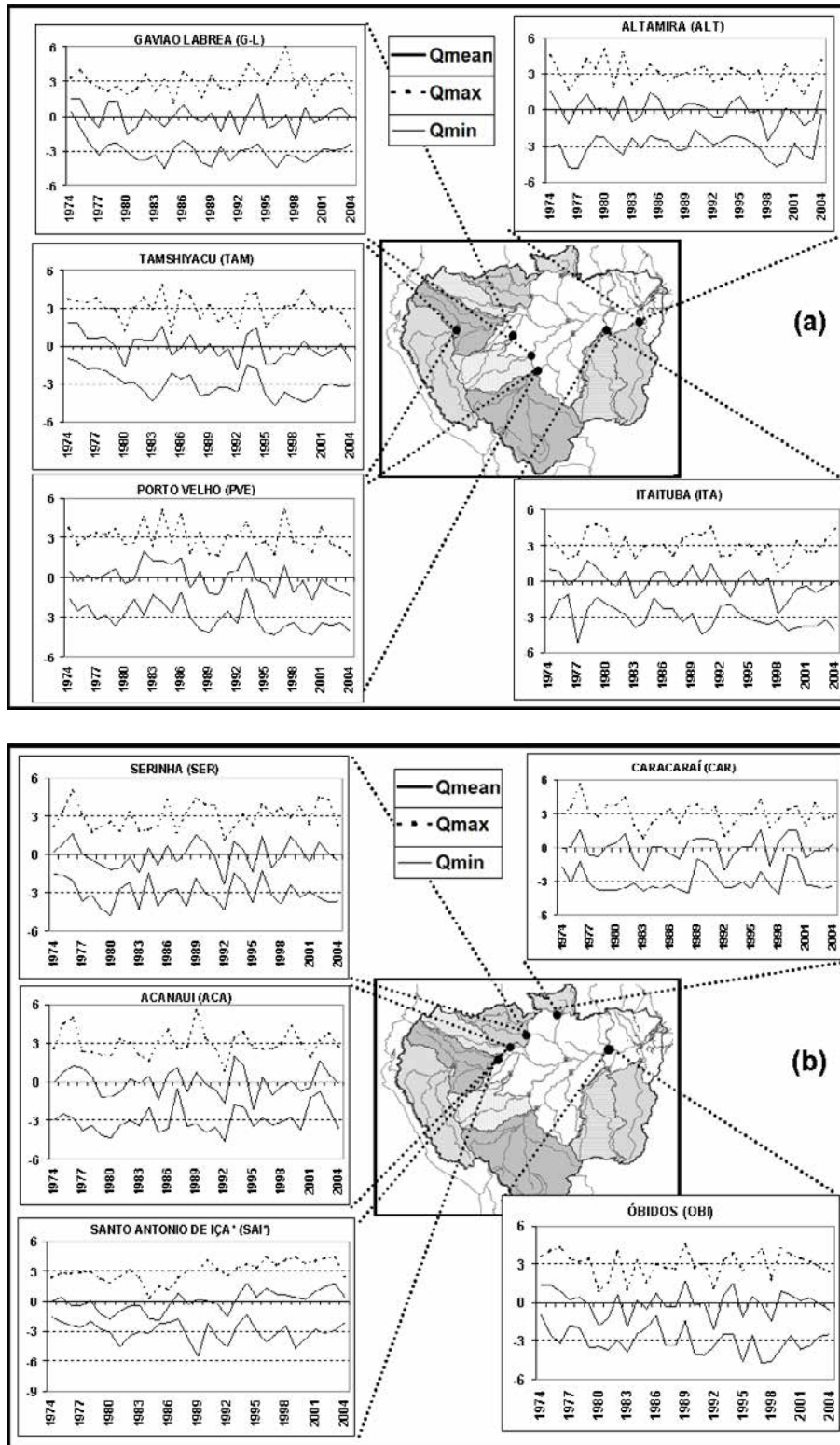
FIGURE 2.4 – Annual Q_{max} , Q_{mean} and Q_{min} time evolution (1974-2004) in a) The southern sub-basins and b) The northern sub-basins of the Amazon. Values are standardized and are corrected by coefficients in order to avoid confusion between the different lines. The coefficient is 3 for Q_{max} , 0 for Q_{mean} and -3 for Q_{min} .
